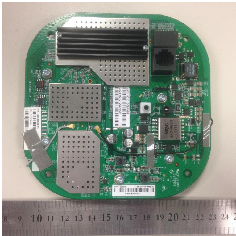
Photo 4 – Main Board Top View
