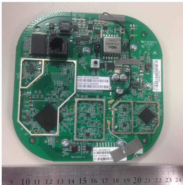
Photo 6 – Main Board Shielding off View
