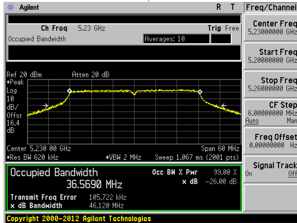
CHAIN 0, 5230 MHz
