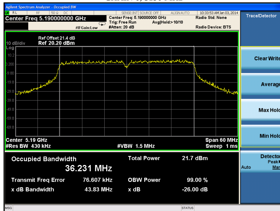
CHAIN 0, 5190 MHz
