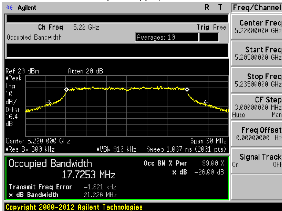
CHAIN 1, 5220 MHz
