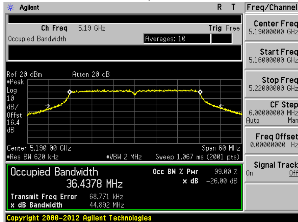
CHAIN 1, 5190 MHz
