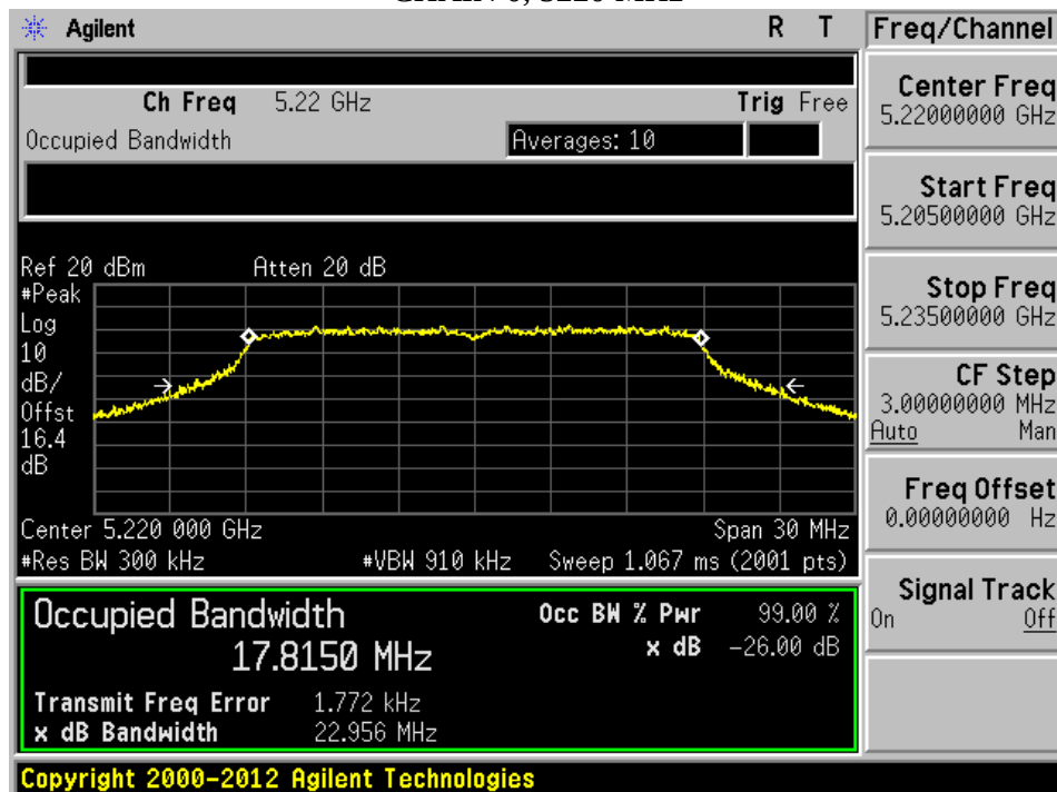
CHAIN 0, 5220 MHz
