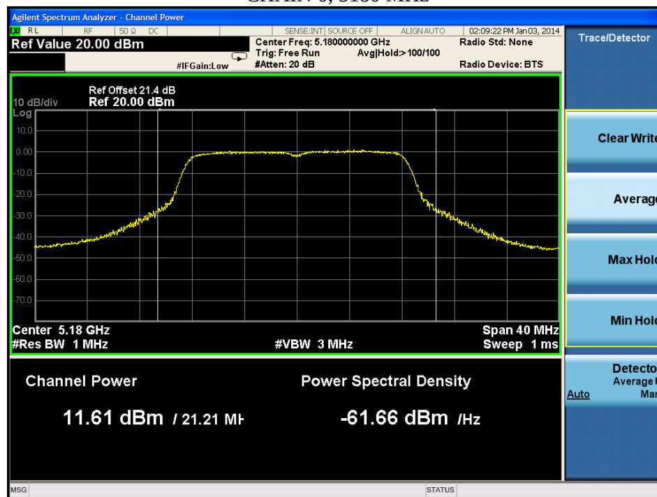
CHAIN 0, 5180 MHz
