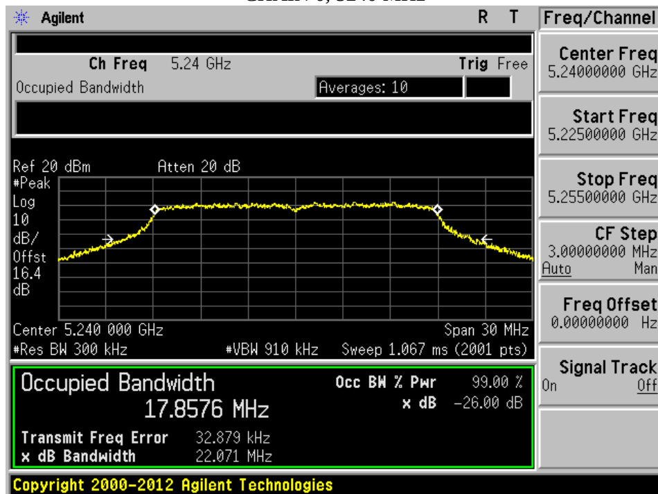
CHAIN 0, 5240 MHz
