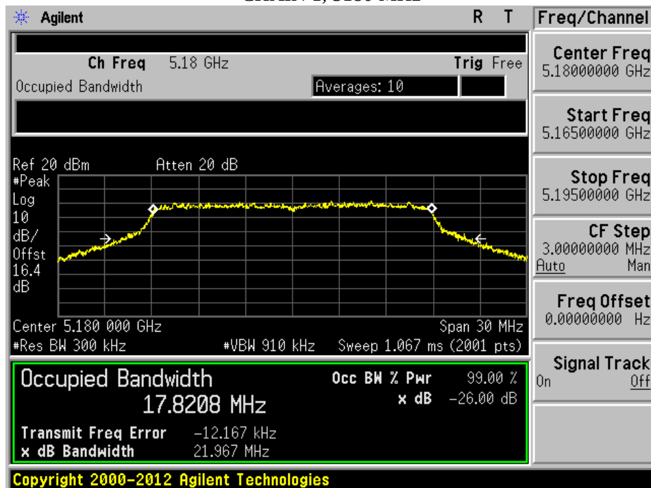
CHAIN 1, 5180 MHz
