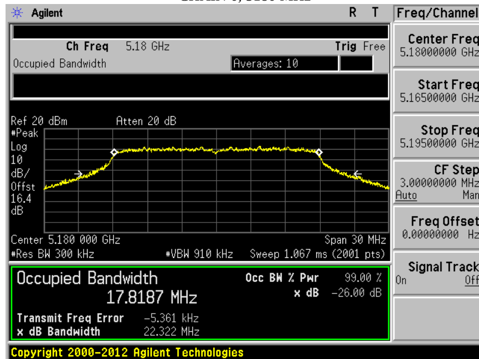
CHAIN 0, 5180 MHz
