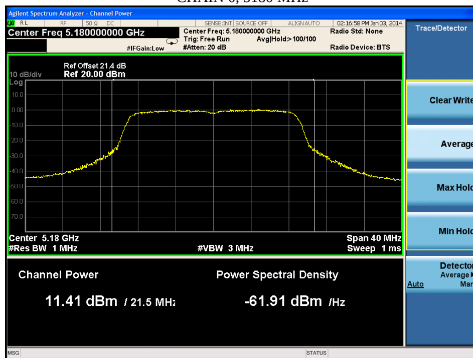
CHAIN 0, 5180 MHz
