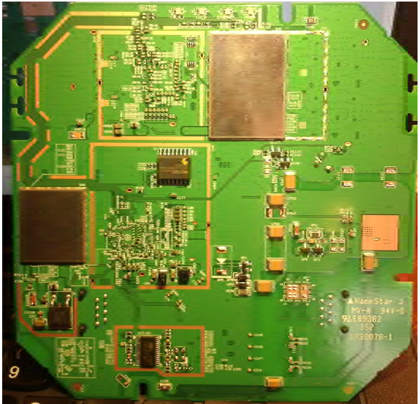
BACK SIDE OF PCB WITH SHIELDS
