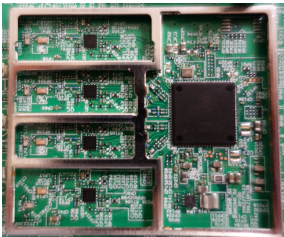
Close-Up – 5GHz Radio
