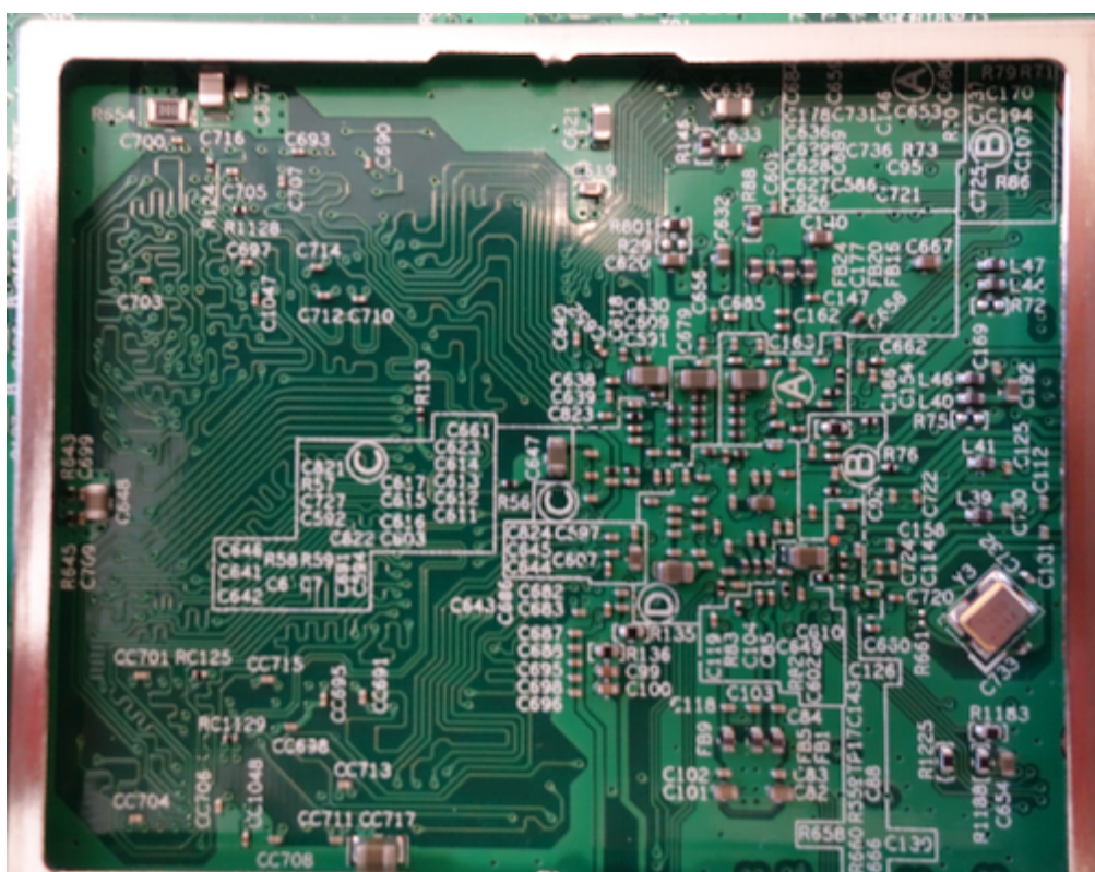
Close-Up CPU Bottom
