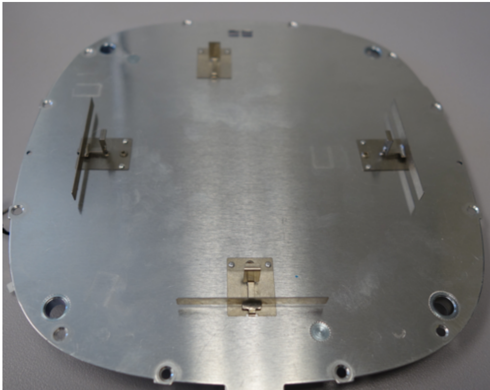
Internal Antenna - Metal Sheet
