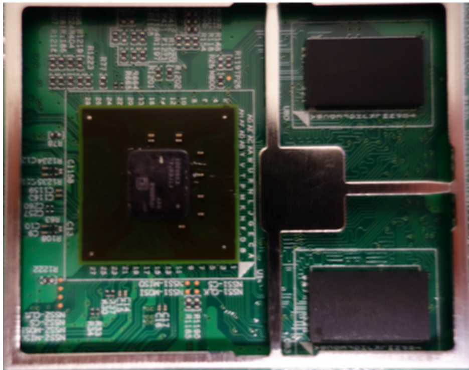
Close-Up – CPU (Shield Removed)
