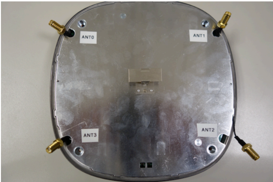
Cover Removed
