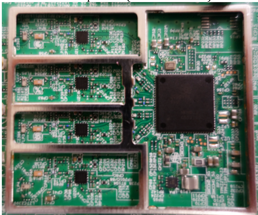
Close-Up – 5GHz Radio
