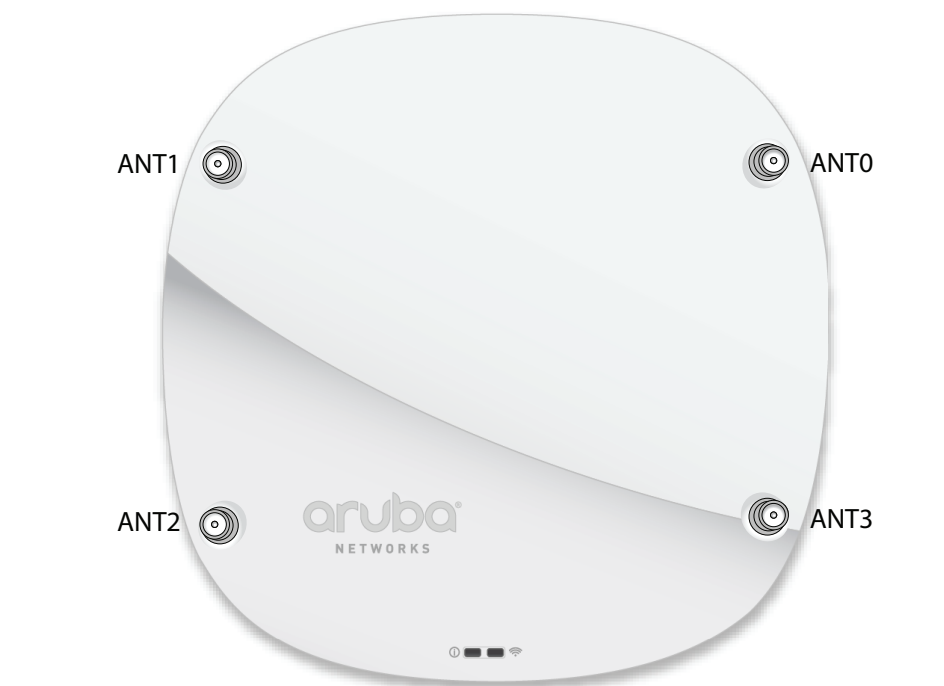
Figure 2 External Antenna Connectors
