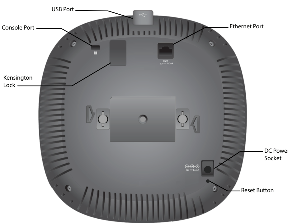
Figure 4 Back Panel
