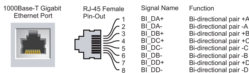
Figure 6 RJ45 Gigabit Port Pin-Out
