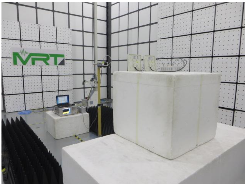
Description: Radiated Spurious Emission Test Setup for 18GHz ~ 40GHz (AP-ANT-48)
