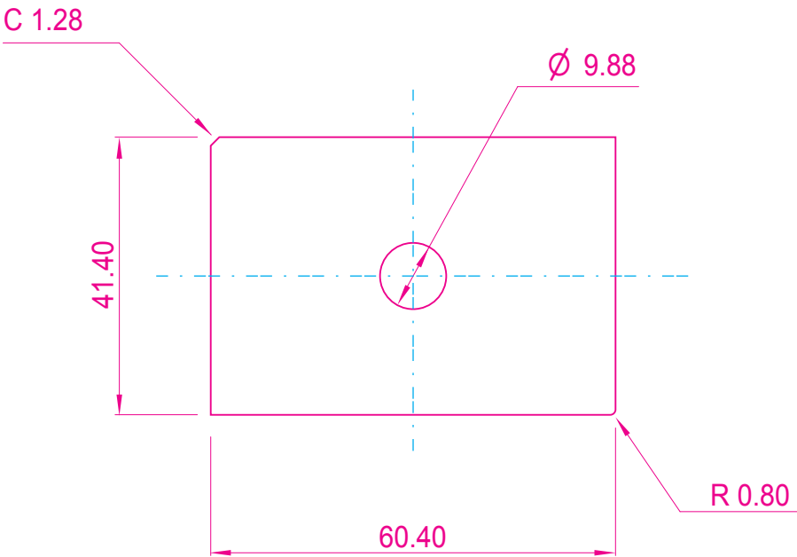
FRONT
