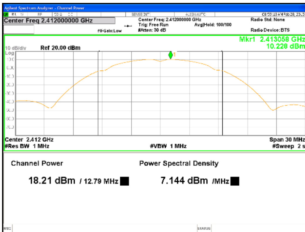
Figure 1: Maximum Transmitted Power, 2412MHz b mode at 1Mbps, Chain 0
