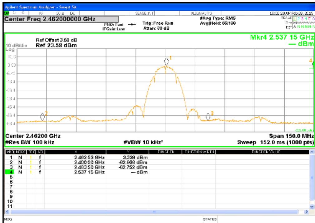
Figure 25: Reference Level for B mode at 2462MHz, Chain1
