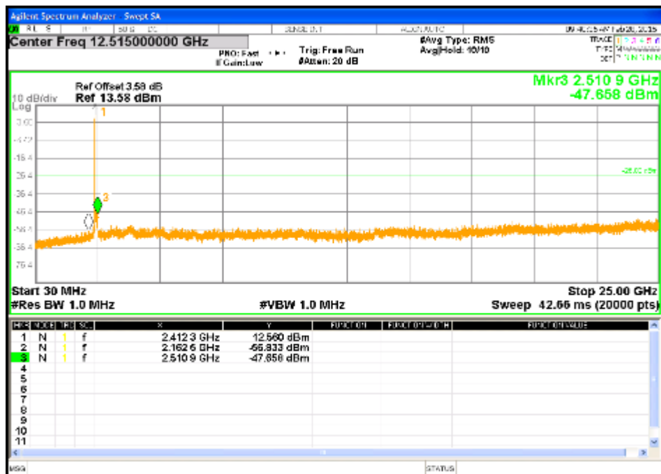
Figure 12: Out of Band emissions b mode 2412MHz, Chain 1
