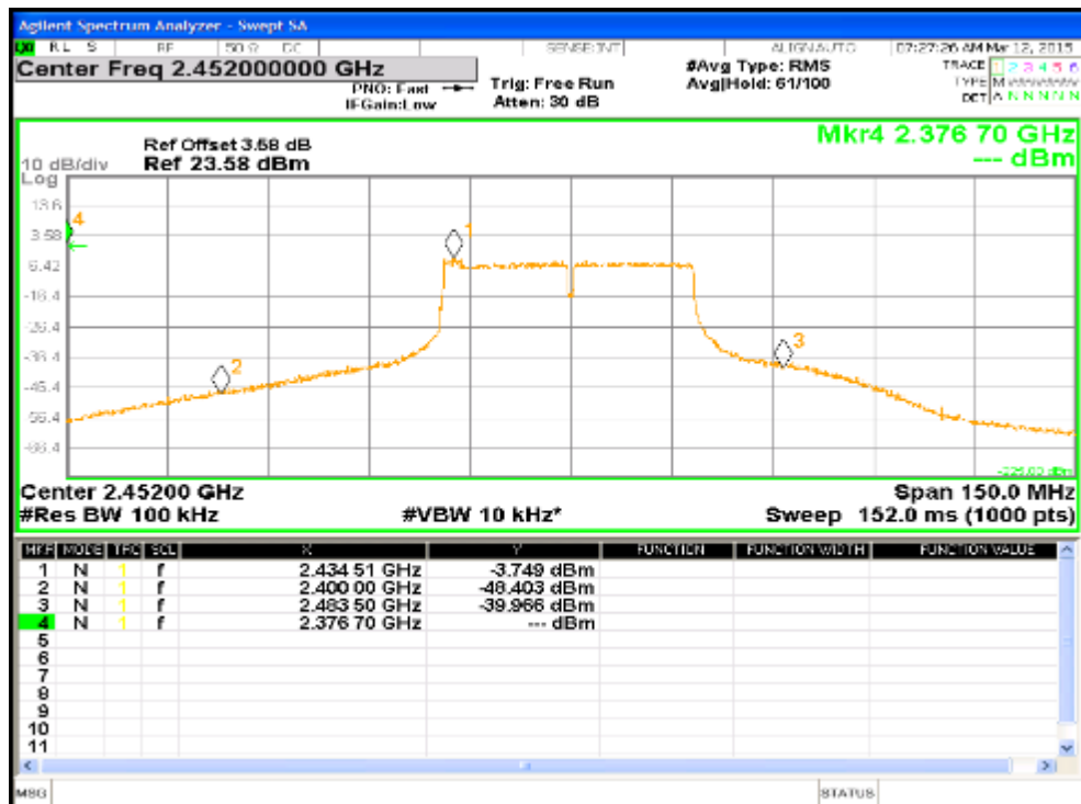
Figure 87: Reference Level for HT40 at 2452 MHz, Chain 0
