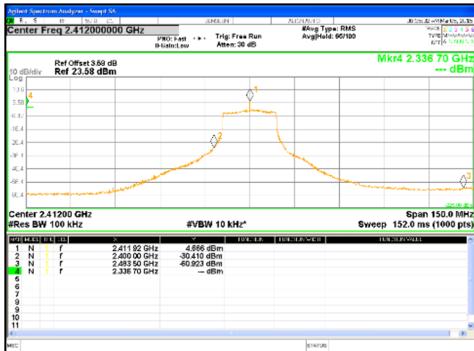
Figure 61: Reference Level for HT20 at 2412MHz, Chain 3
