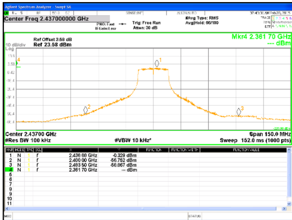
Figure 41: Reference Level for 802.11g mode 2437MHz, Chain1
