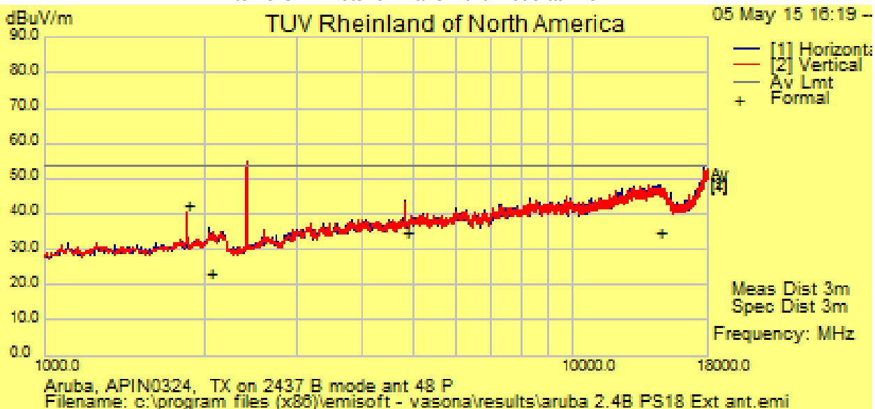
1 to 18 GHz Plots for Transmit b Mode at 2437 MHz
