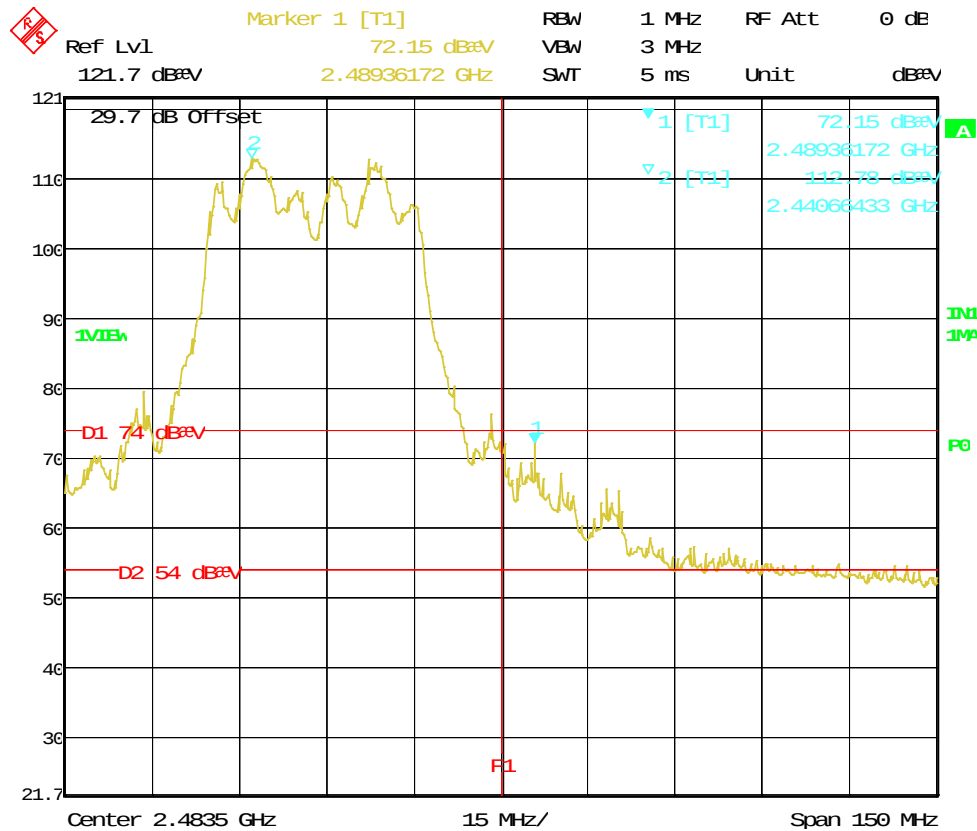
Figure 115: Radiated Emission at the Edge for 2452 MHz HT40- Vert. (Pk)
