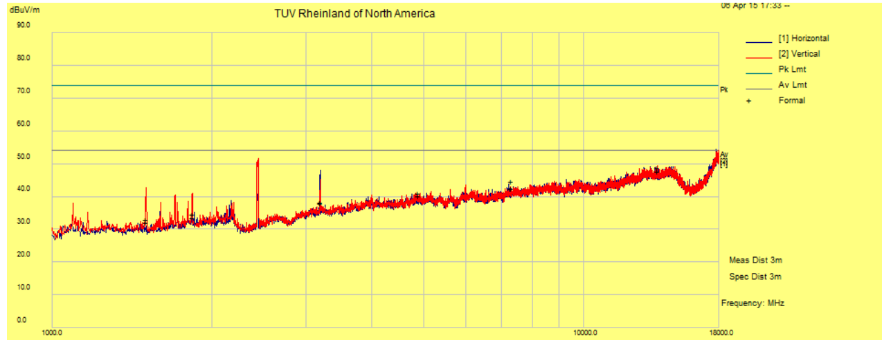
1 to 18 GHz Plots for Transmit Mode b at 2437MHz
