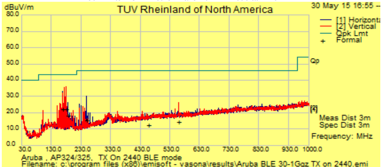
30MHz to 1 GHz Plot for Transmit BLE Mode at 2440MHz
