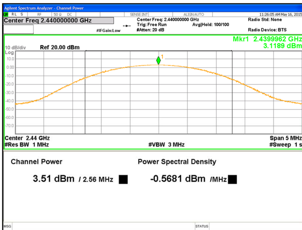
Figure 2: Maximum Transmitted Power, 2440MHz BLE mode at 1Mbps
