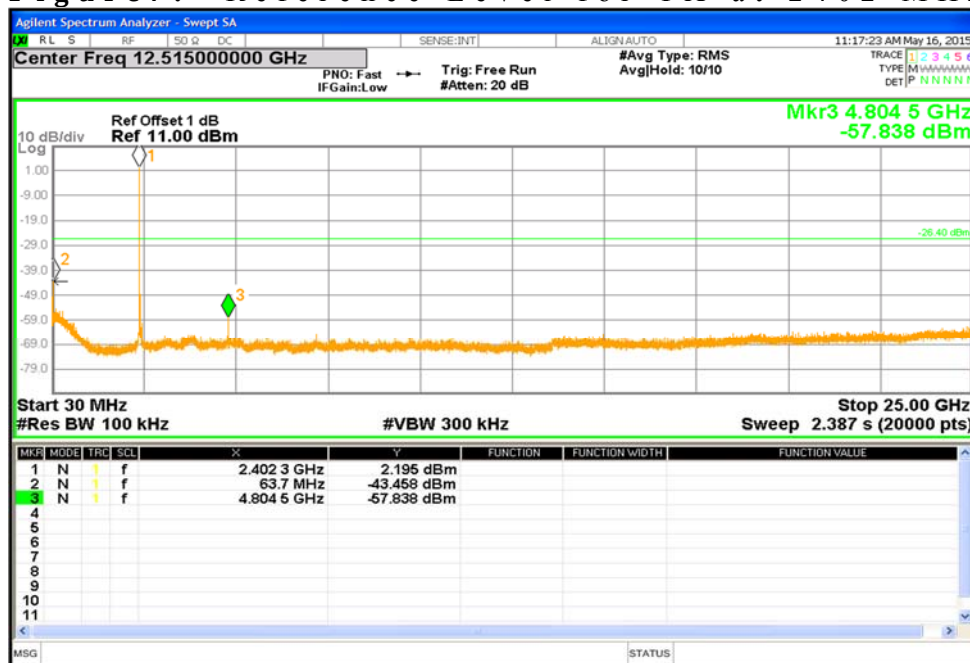
Figure 8: Out of Band Emission for TX at 2402 MHz
