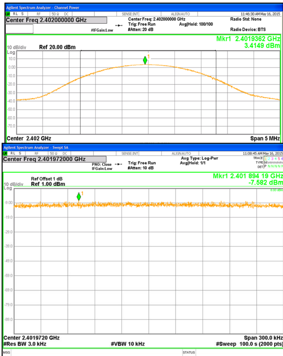
Figure13: PSD, 2402MHz, BLE mode at 1Mbps (Close up plot)
