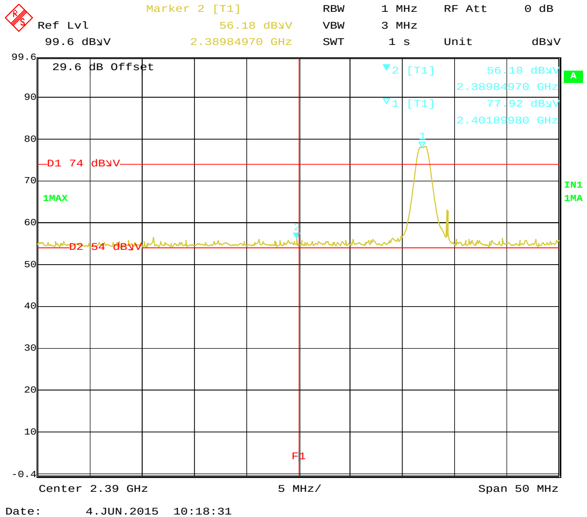
Figure 16: Radiated Emission at the Edge for 2402 MHz –Vert. (Pk)
