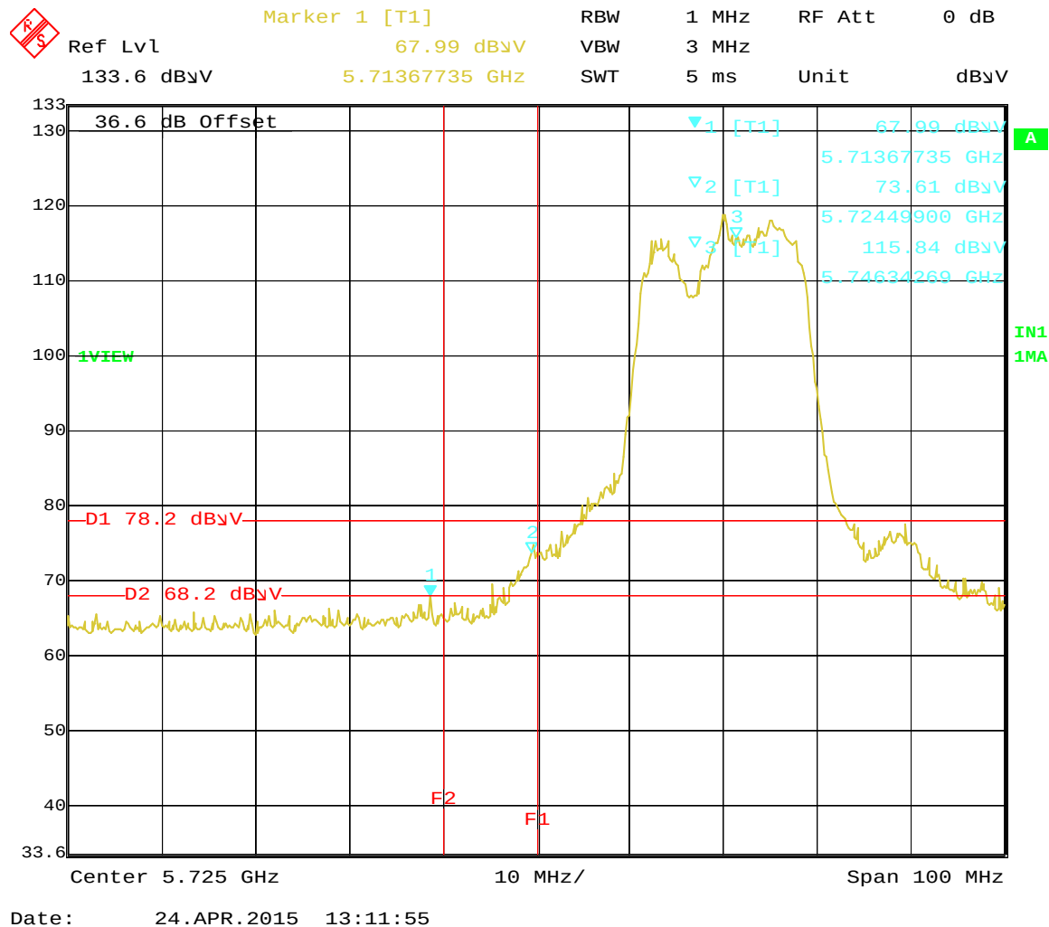
Figure 29: Radiated Emission at the Band Crossing for Channel 5745 MHz at HT20 6.5Mbps – Vert. (Ave.)
