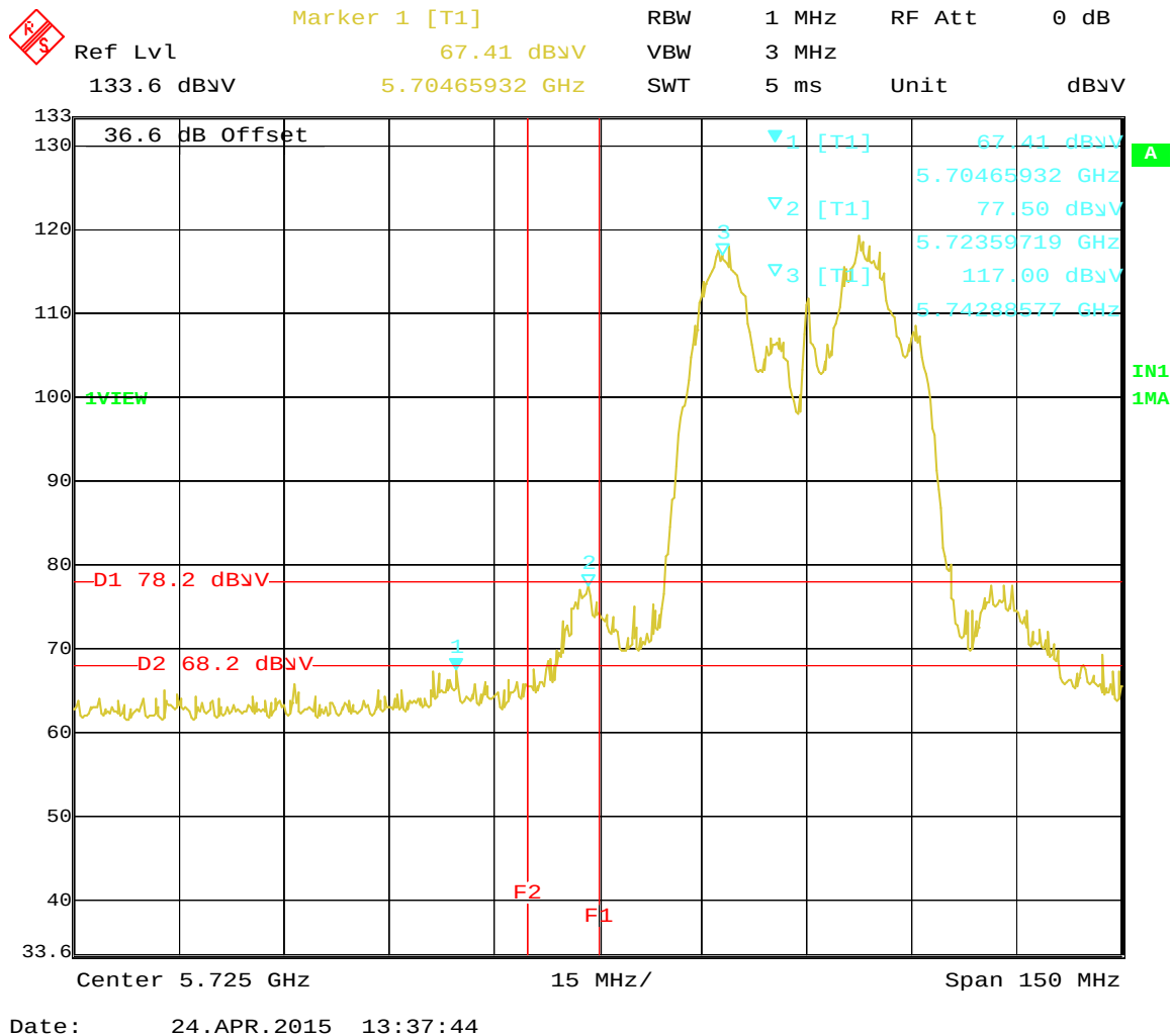
Figure 30: Radiated Emission at the band crossing for TX 5755Hz at HT40 at 13.5.5Mbps– Vert. (Peak)
