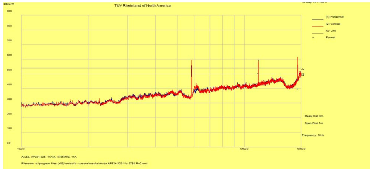
1 -18 GHz Plot for Transmit Mode at 5785 MHz
