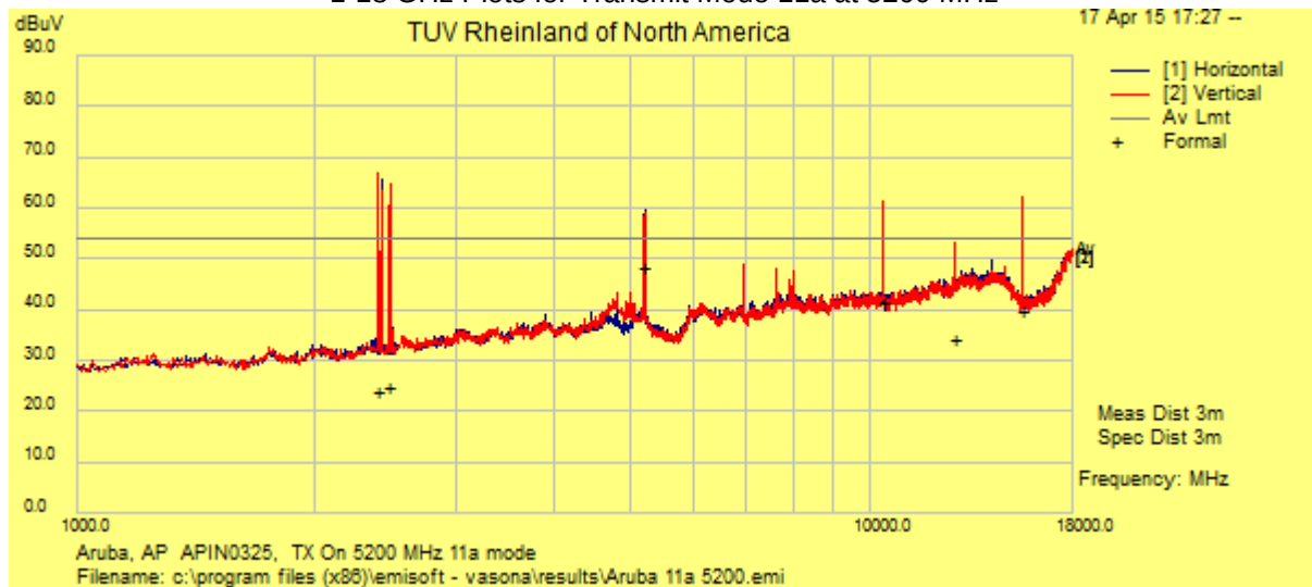
1-18 GHz Plots for Transmit Mode 11a at 5200 MHz
