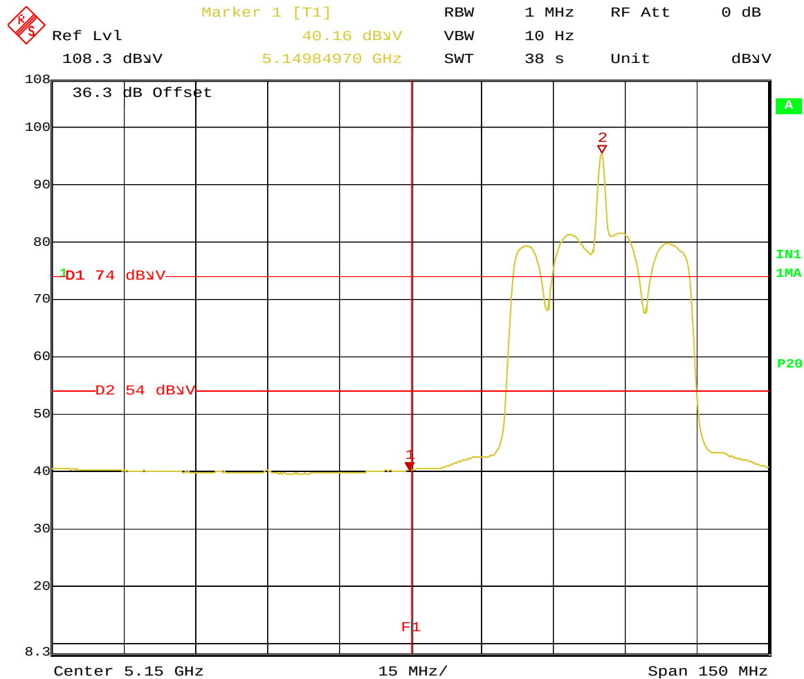
Figure 37: Radiated Emission at the Edge for 5190 MHz at HT40 13.5Mbps – Horiz. (Avg)
