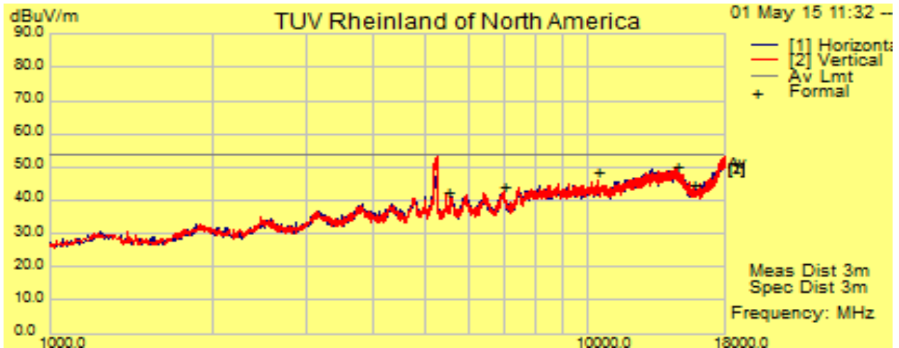
1 -18 GHz Plot for Transmit Mode at 5210 MHz
