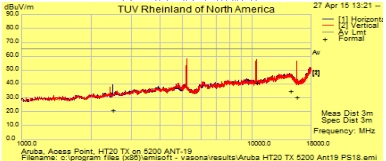
1 -18 GHz Plot for Transmit Mode at 5200 MHz
