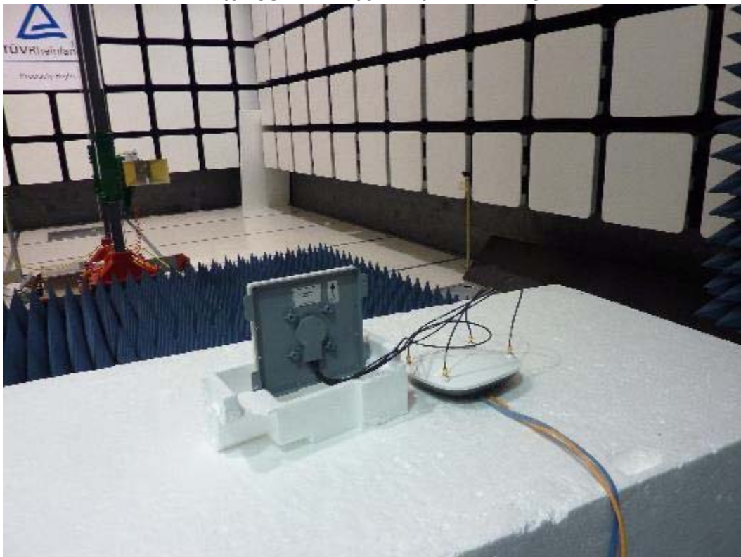
1 to 18GHz APIN0324 with AP-ANT-48
