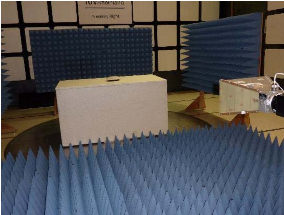
1 to 18GHz APIN0325
