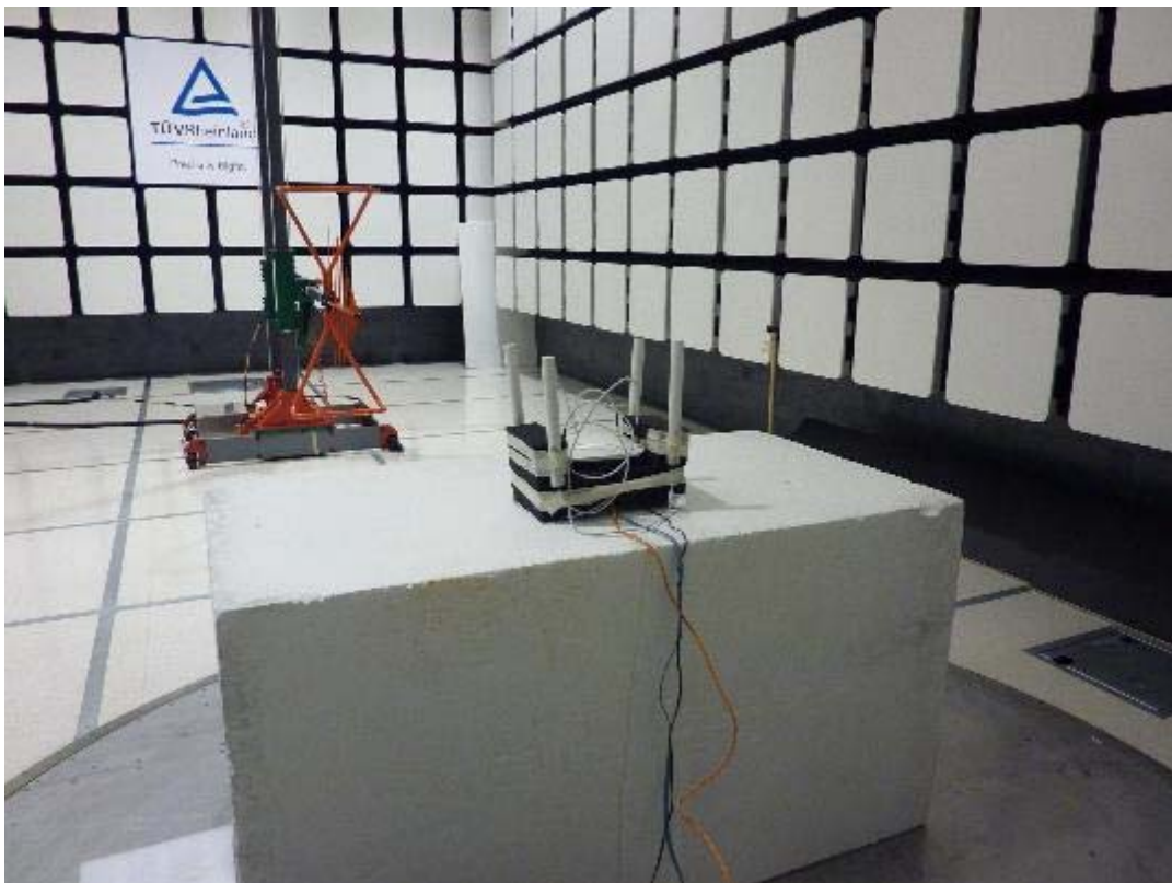
30 to 1000MHz APIN0324
