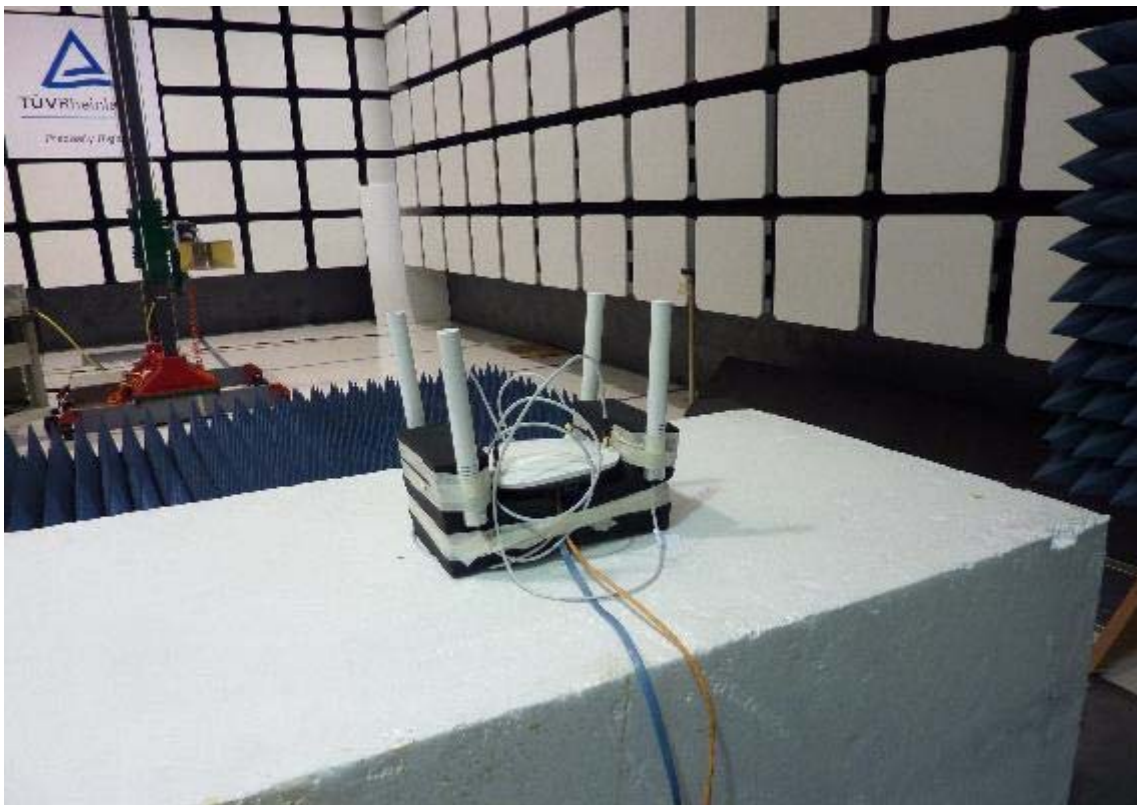
1 to 18GHz APIN0324 with AP-ANT-19
