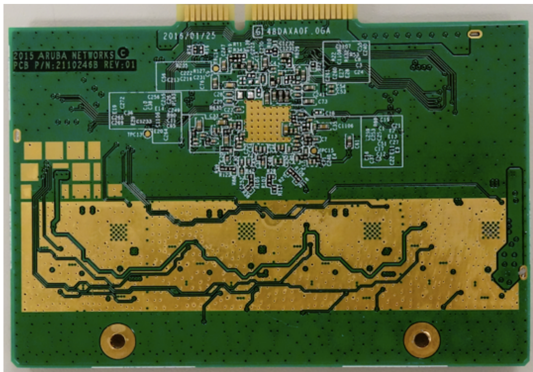
Bottom view of 5GHz Radio Card
