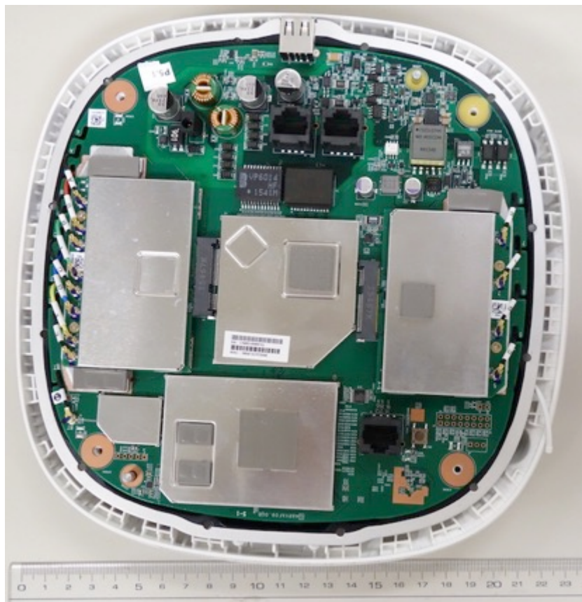
Metal Plane Removed
