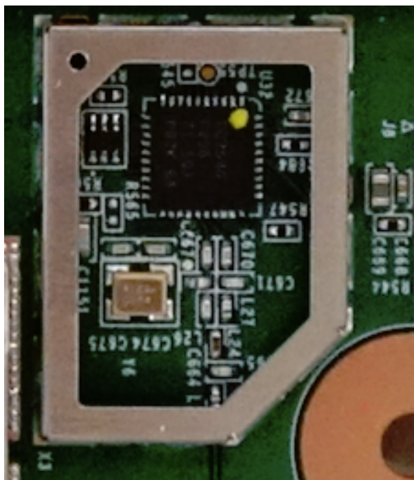
Close-up of BLE with Shield Removed
