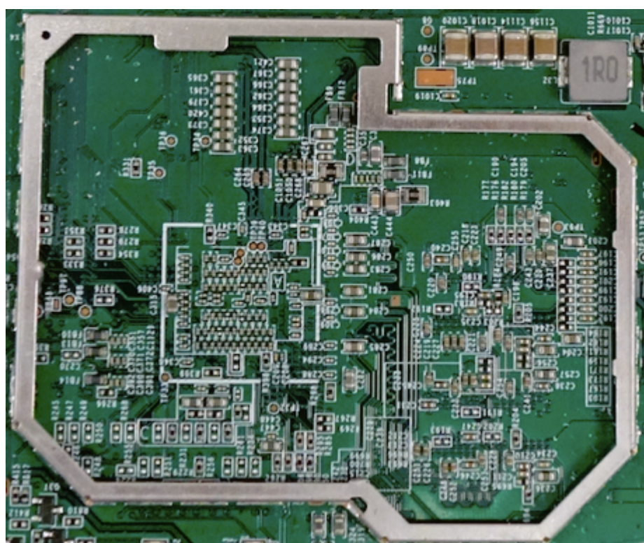
Close-Up with Shield Removed
