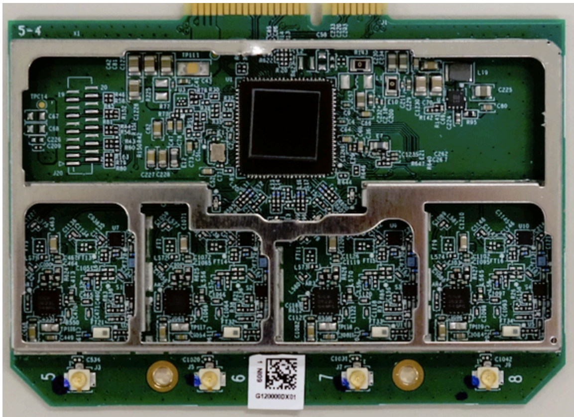
Close-up of 5GHz RF Card with Shield Removed
