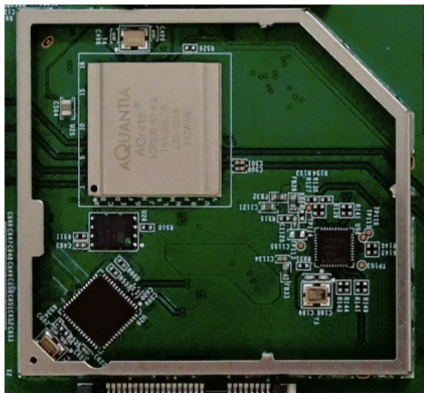
Close-Up with shield removed
