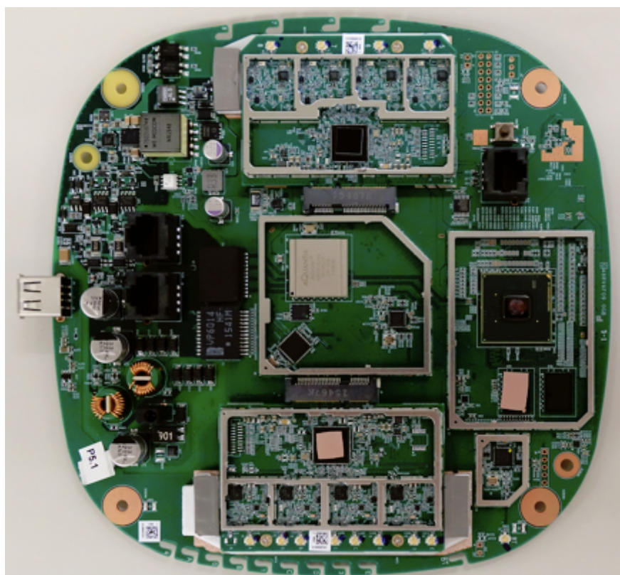
PCB - Top with Shields Removed
