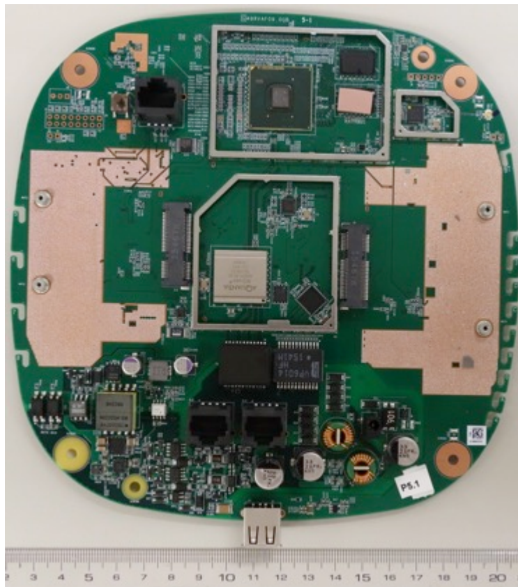
PCB Top – RF Cards Removed
