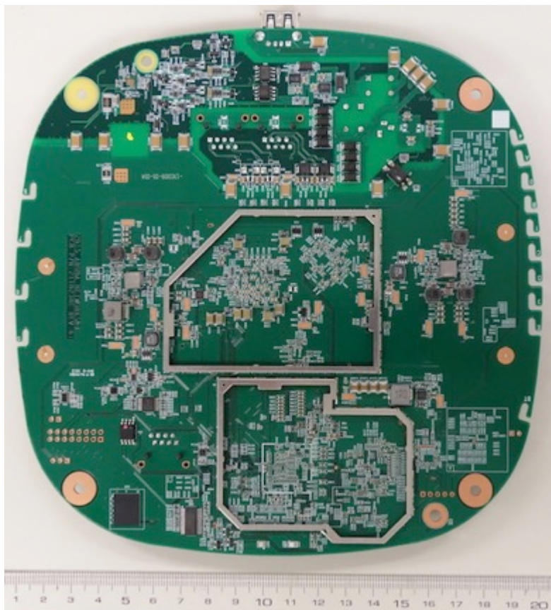
PCB - Bottom with Shield Removed
