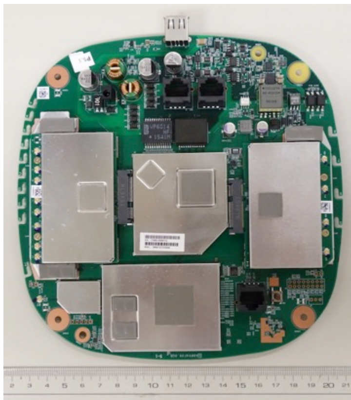
PCB - Top View
