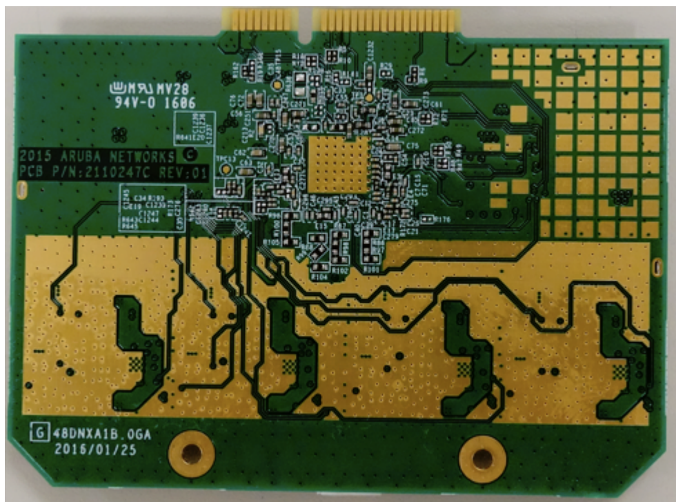
2.4GHz Radio – Bottom View
