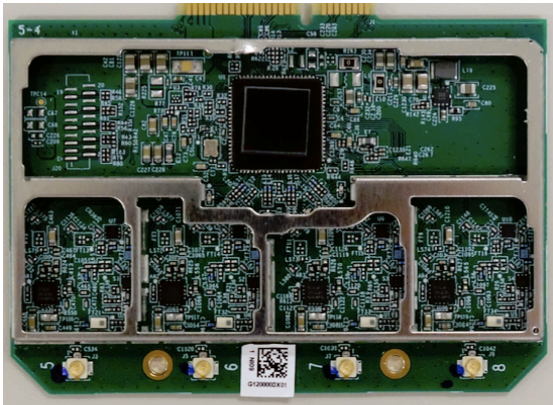
Close-up of 2.4GHz Radio with Shield Remove
