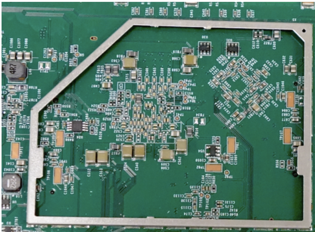
Close-Up with Shield Removed
