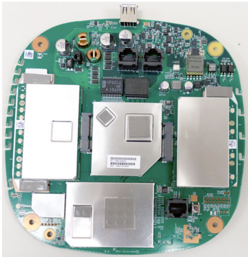
Top View of PCB
