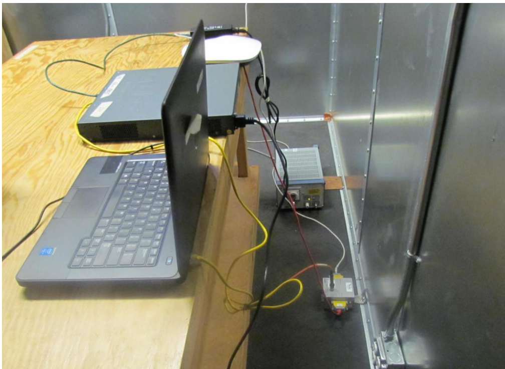
PoE Configuration – Signal Line Rear View
