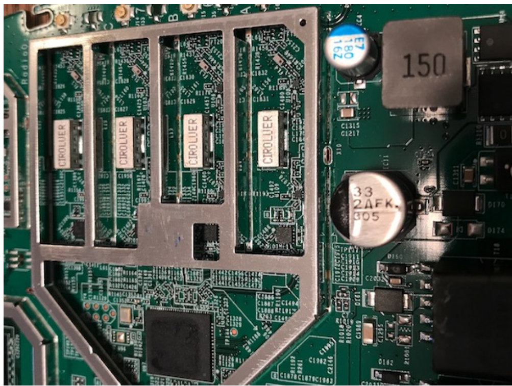
Close-Up: Radio 1
