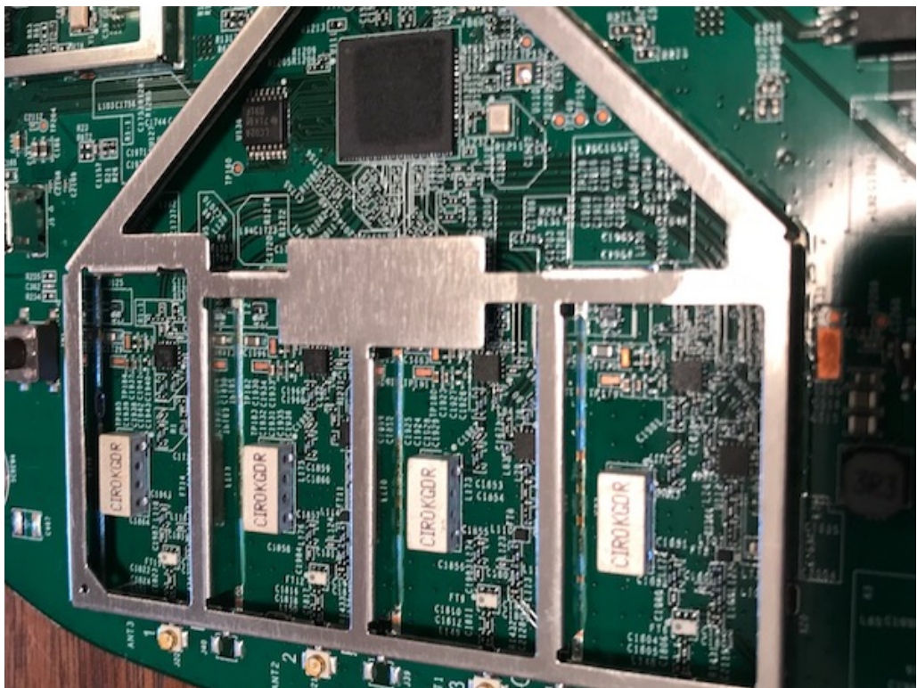
Close-Up: Radio 0
