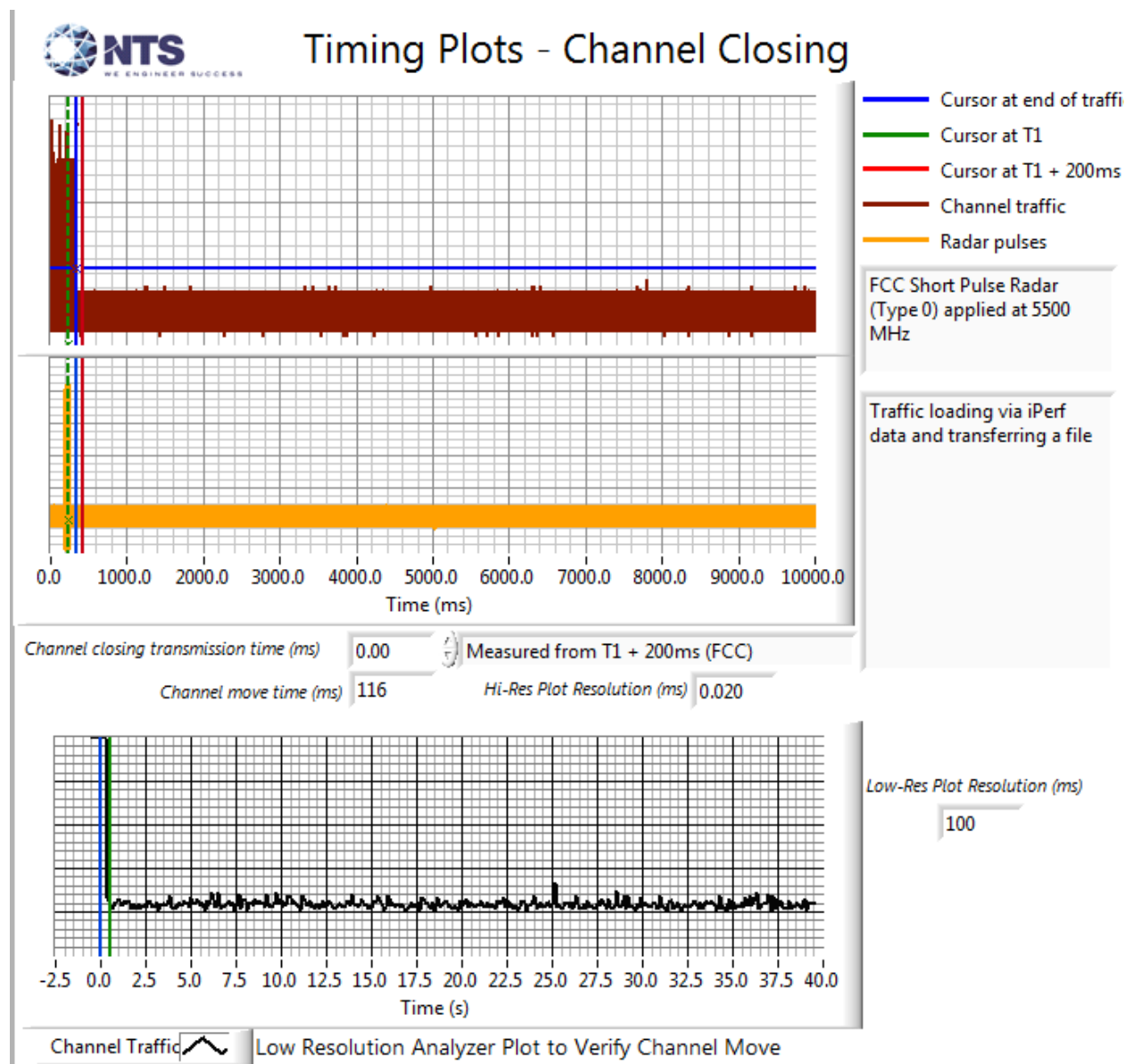
Figure 12 Channel Closing & Channel Move Time (80+80MHz) UNIL-2C plot
