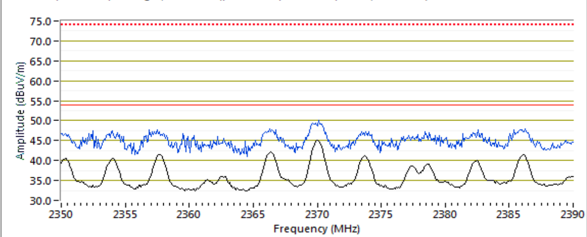
RB 1 MHz; VB 3 kHz; Average (Black Trace); RB 1 MHz; VB 3 MHz; Peak (Blue Trace)
