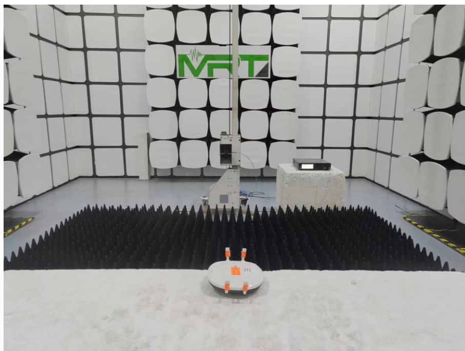
Description: DFS Test Setup
