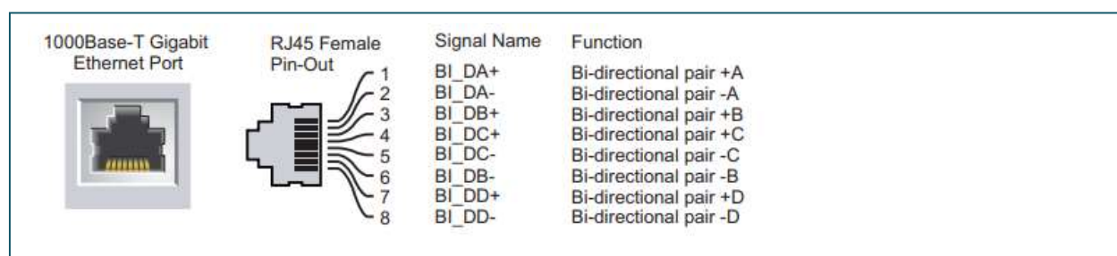
Figure 10 100/1000/2500/5000 Base-T
