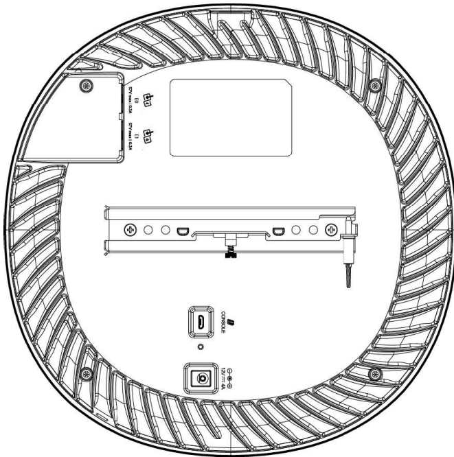
Figure 8 AP-654 Access Point Rear View
