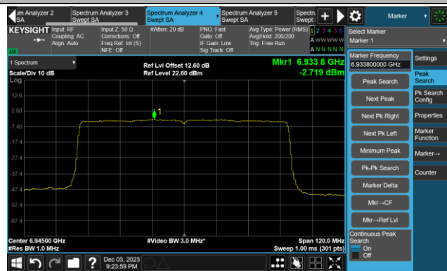
Channel 199 (6945 MHz)
