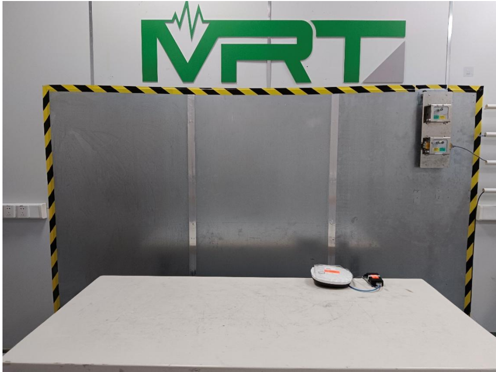
Description: Side View of AC Power Conducted Emission Test Setup
