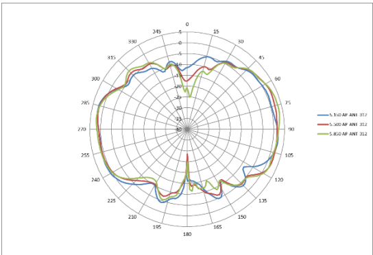
5GHz antennas patterns (vertical/90)
