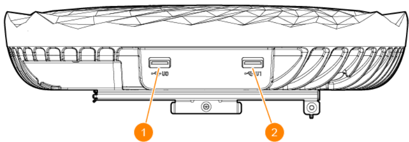
Figure 3 AP-755 Access Point Side A View
