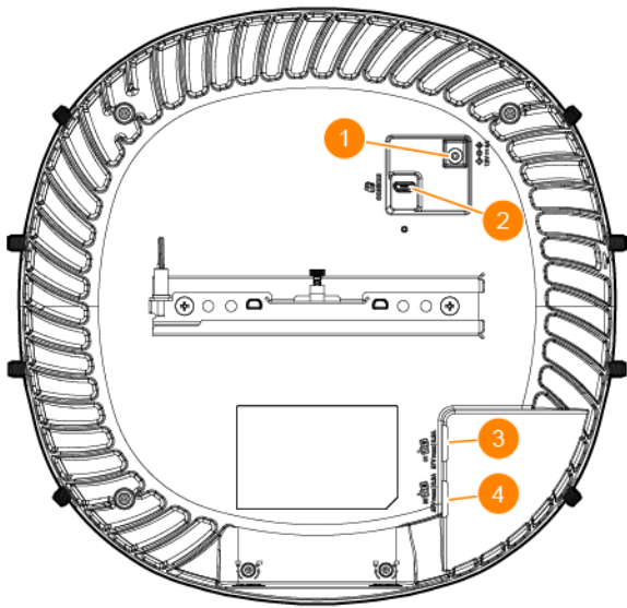
Figure 8 AP-754 Access Point Rear View
