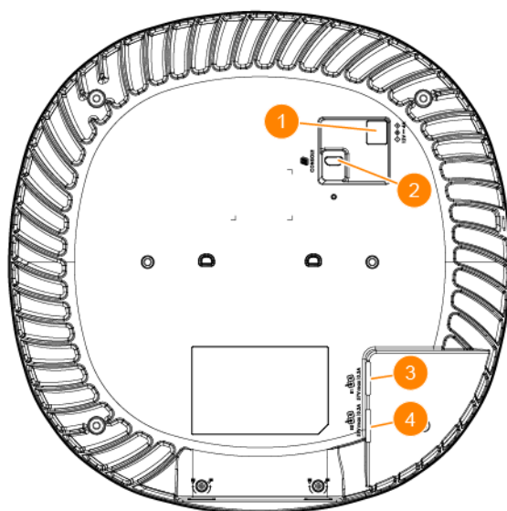
Figure 7 AP-755 Access Point Rear View
