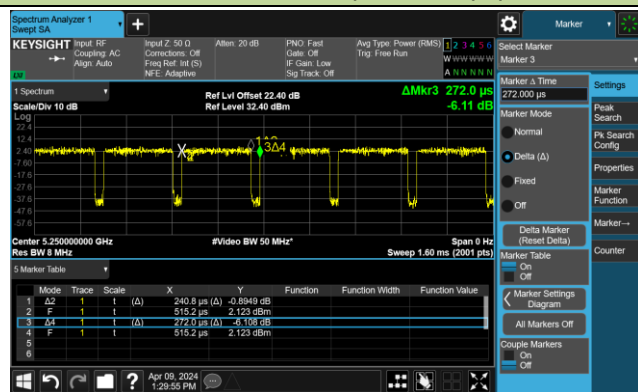
802.11be-EHT40 (T = 772.7µs)
