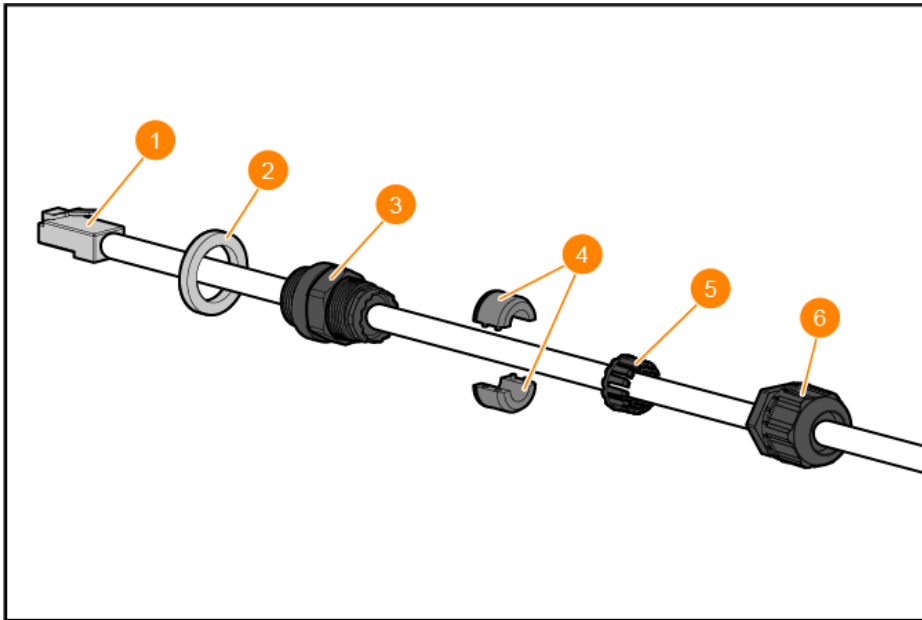
Figure 20 Ethernet Cable and M20 Cable Gland Assembly
