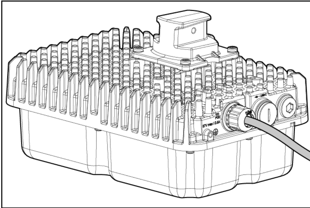
Figure 21 Ethernet Cable and M20 Cable Gland installed to AP
