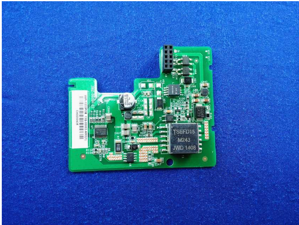
POE Board
