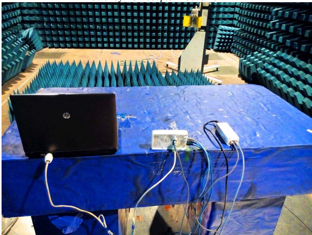
Power by POE adaptor Above 1GHz
