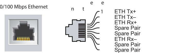
Figure 5 Fast Ethernet Port Pin-Out
