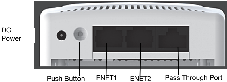
Figure 3 Bottom
