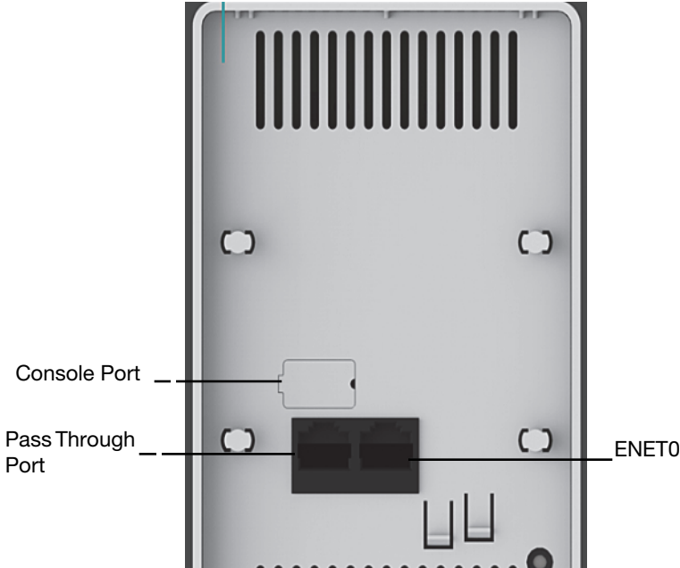
Figure 2 Rear
