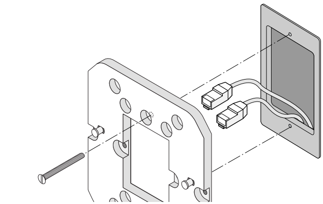
Figure 7 Bracket to Gang Box (Standard US Single Gang Outlet Box Shown)
