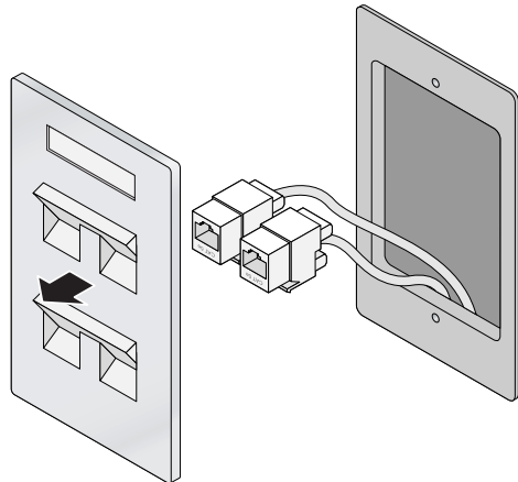
Figure 6 Removing Wall Plate (Standard US Single Gang Outlet Box Shown)
