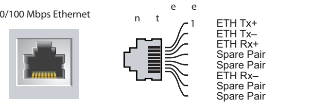
Figure 5 Fast Ethernet Port Pin-Out
