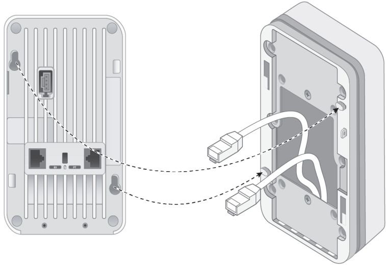
Figure 8 Attaching AP-205H to Bracket
