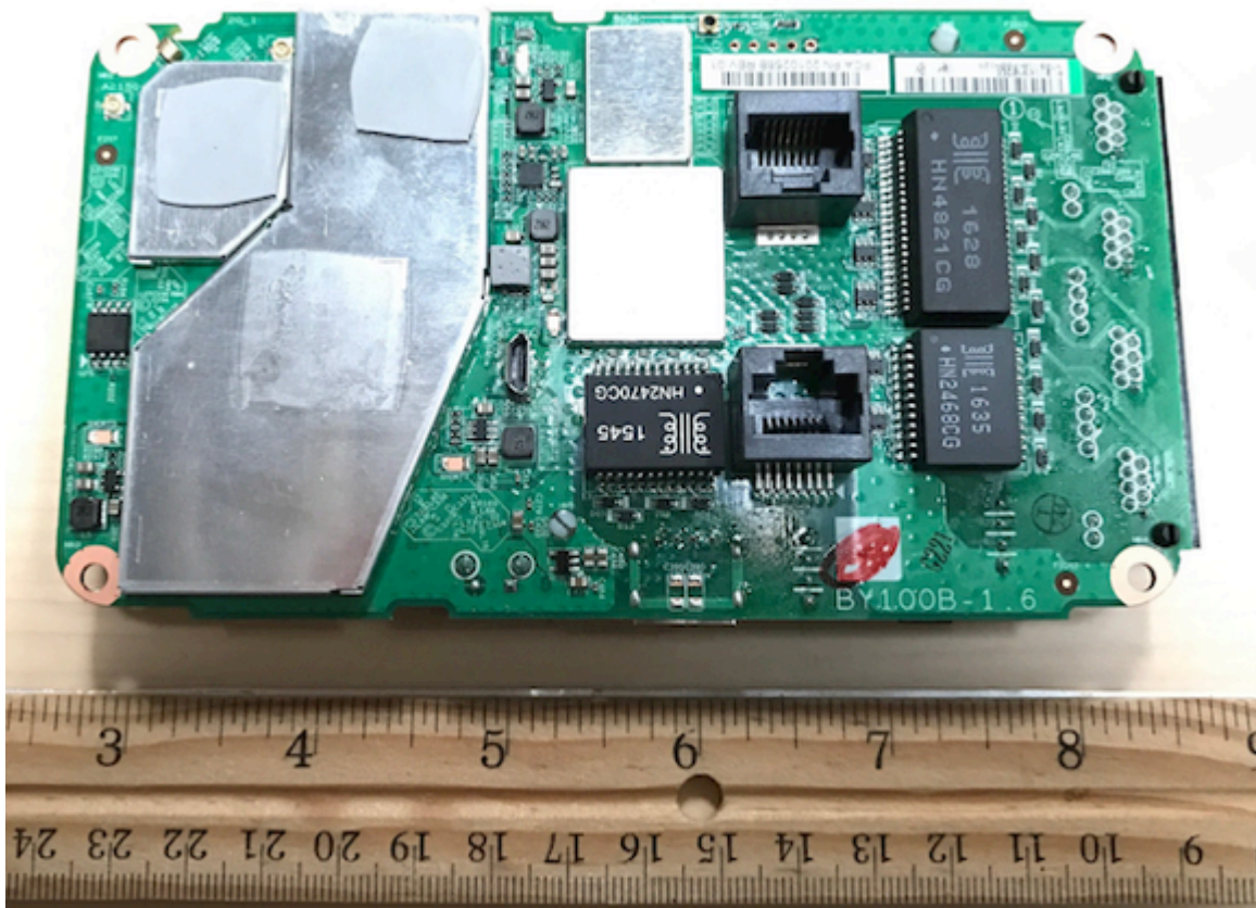
Rear Housing Removed
