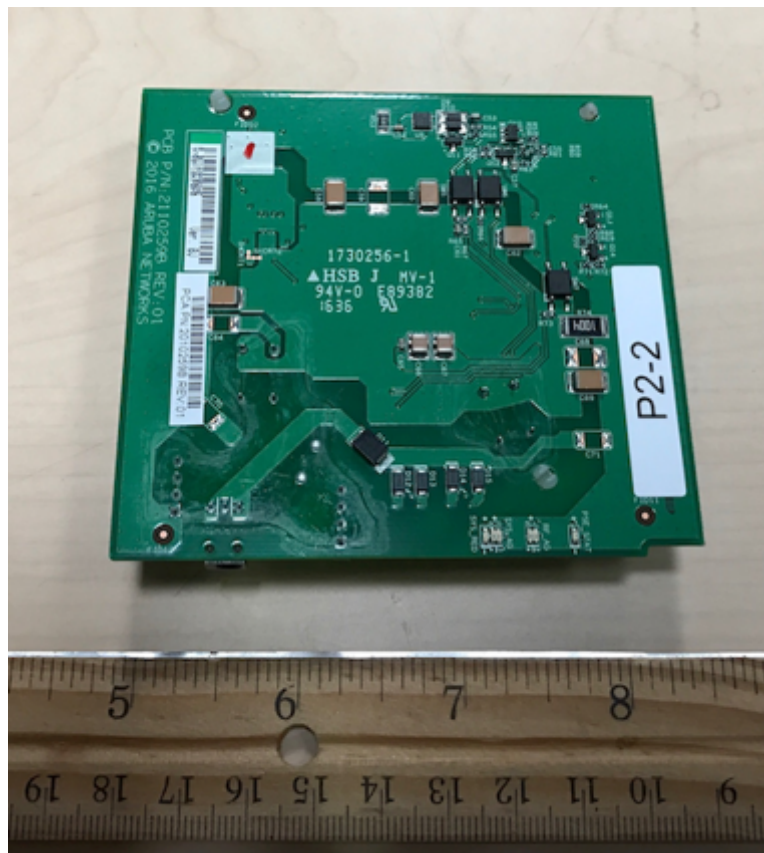
Bottom - Power Board
