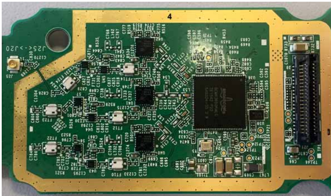
Close-up of Bottom Section Marked 4 – 5GHz Radio
