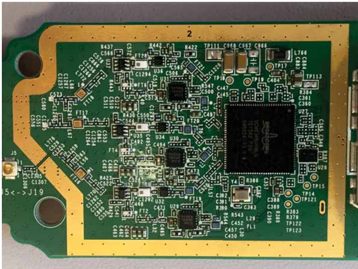
Close-up of Bottom Section Marked 2 – 2GHz Radio
