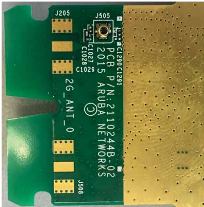
Close-Up of Section Marked 1 – Antenna Ports
