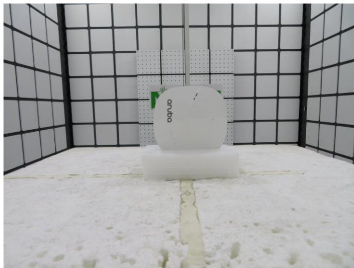
Description: EUT Orientation - Z Axis
