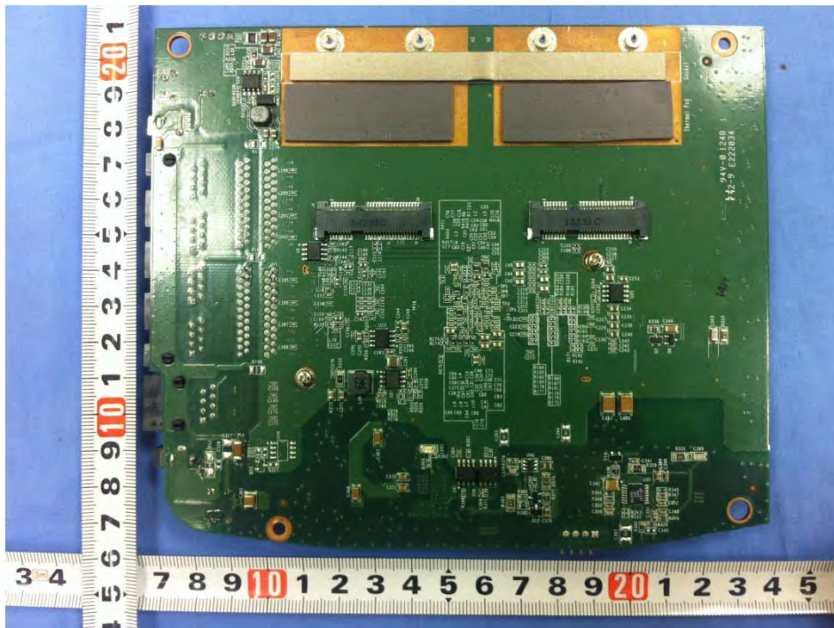
Photo 10– APINR15P Main Board Back View
