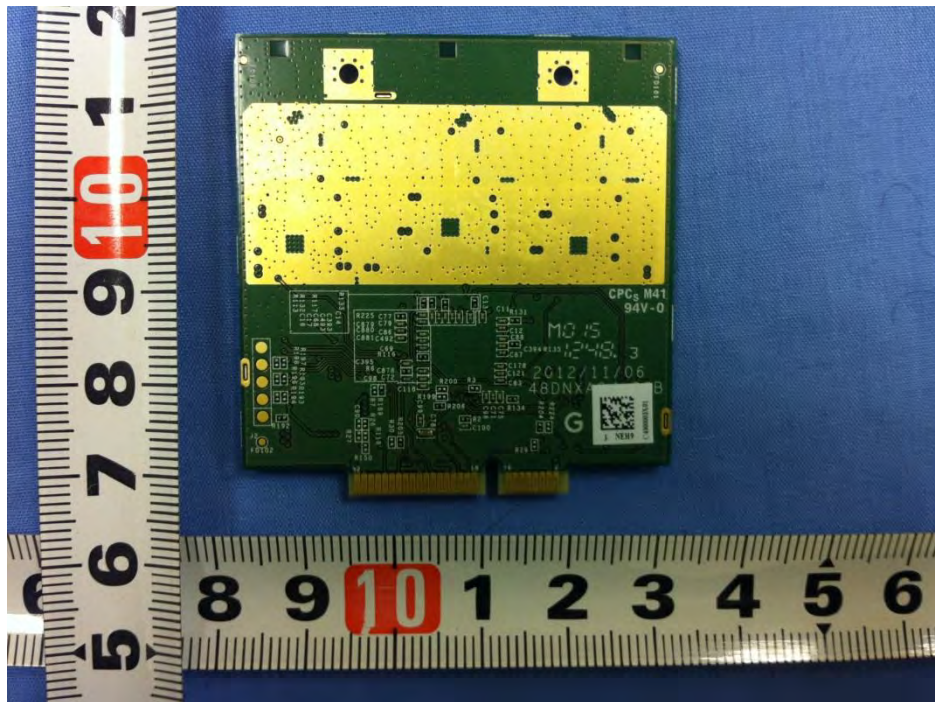
Photo 12– APINR15P 2.4 GHz Radio back View
