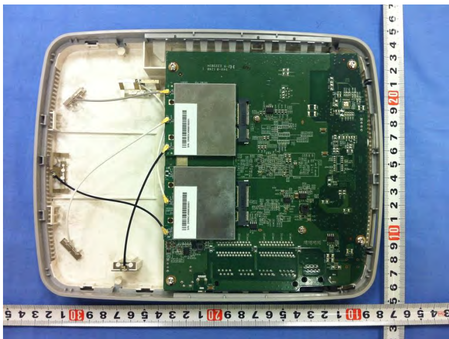
Photo 1 – APINR155 Open Cover View
