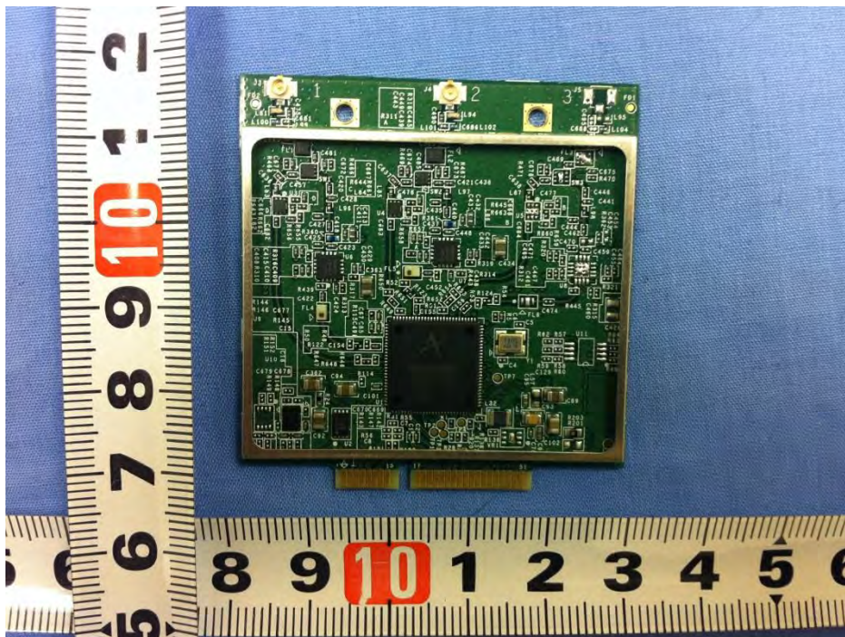
Photo 10– APINR15P Main Board Back View
