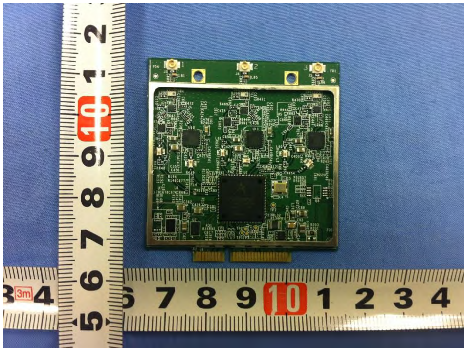
Photo 6 – APINR155 5 GHz Radio Front View
