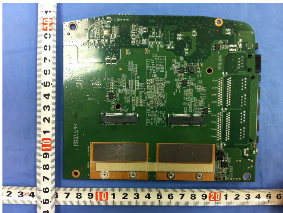
Photo 3– APINR155 Main Board Back View
