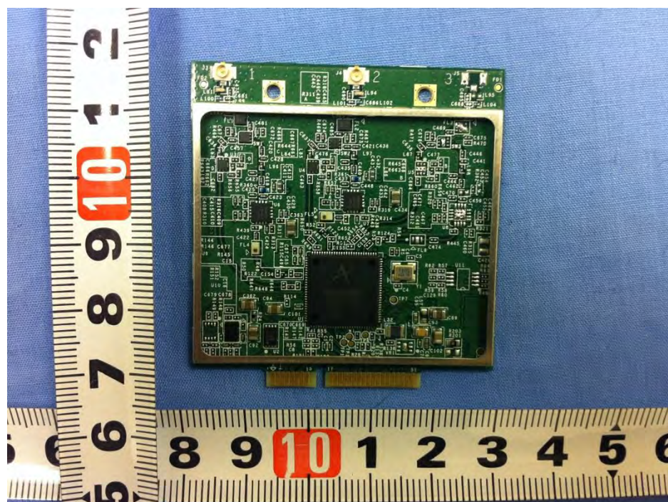
Photo 3– APINR155 Main Board Back View
