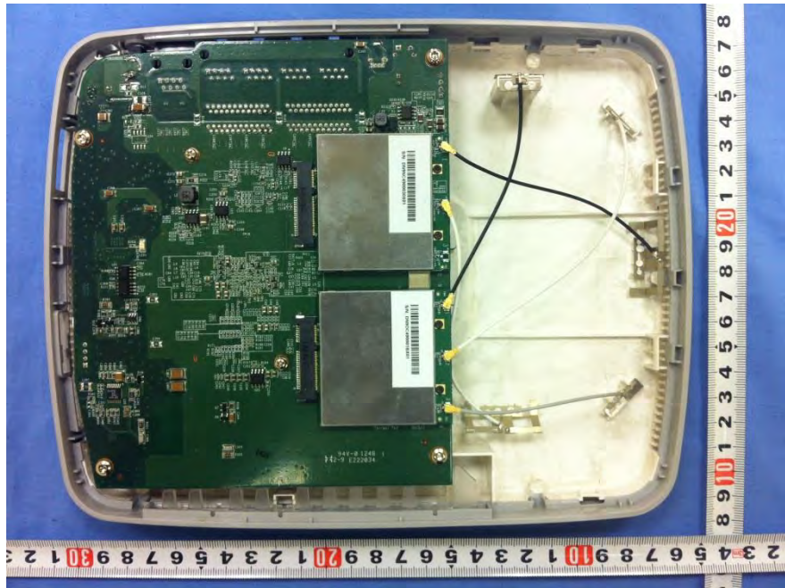
Photo 8 – APINR15P Open Cover View
