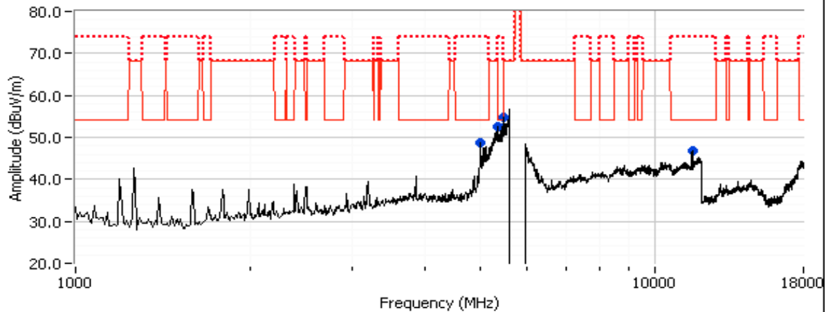
5785 MHz, 802.11a
