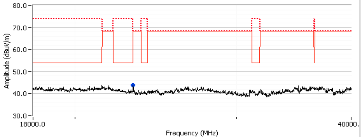
5785 MHz, 802.11a
