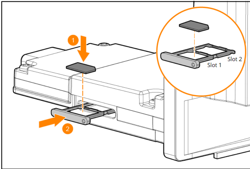
Figure 9 Inserting a SIM Card
