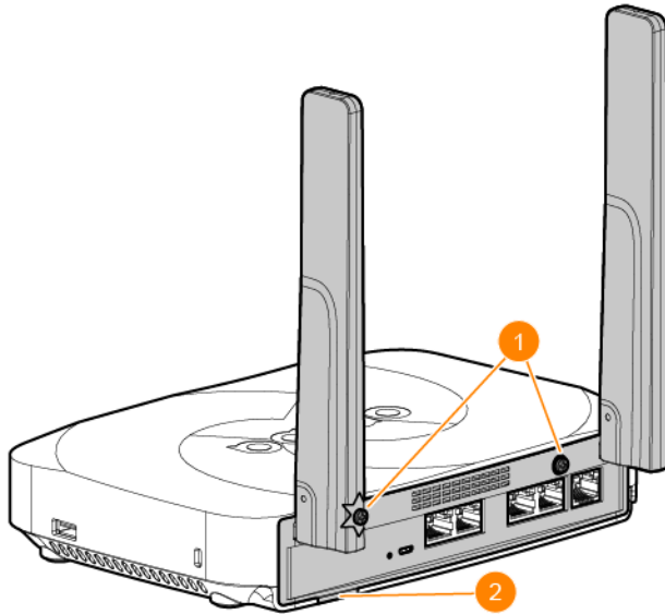
Figure 7 Removing Cellular Module from the Access Point
