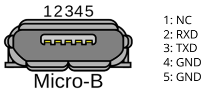
Figure 4 Micro-B Console Port Pin-out
