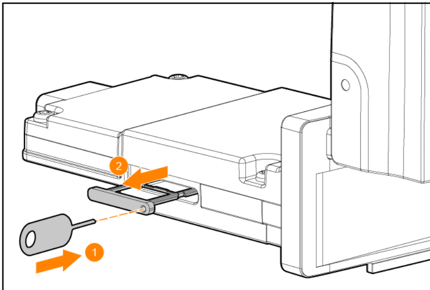
Figure 8 Opening the SIM Card Tray
