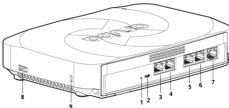
Figure 3 605R Series Rear and Side View
