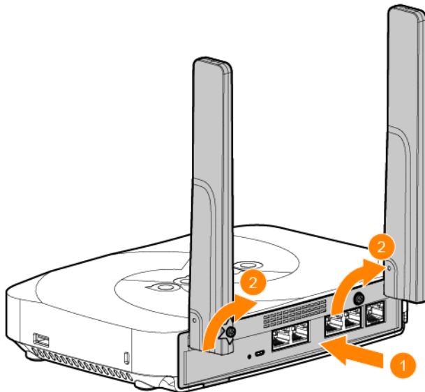
Figure 10 Installing Cellular Module onto Access Point
