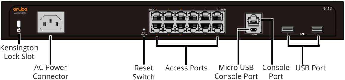
Figure 2 Back Panel of the Aruba 9012 gateway
