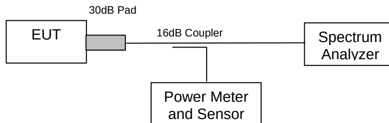
Measurement set up for Transmitter Output Power
