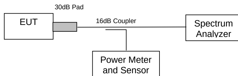
Measurement set up for 6dB Bandwidth test
