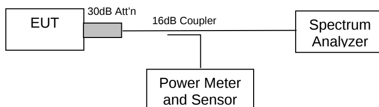
Measurement set up for 26dB/99% Bandwidth test
