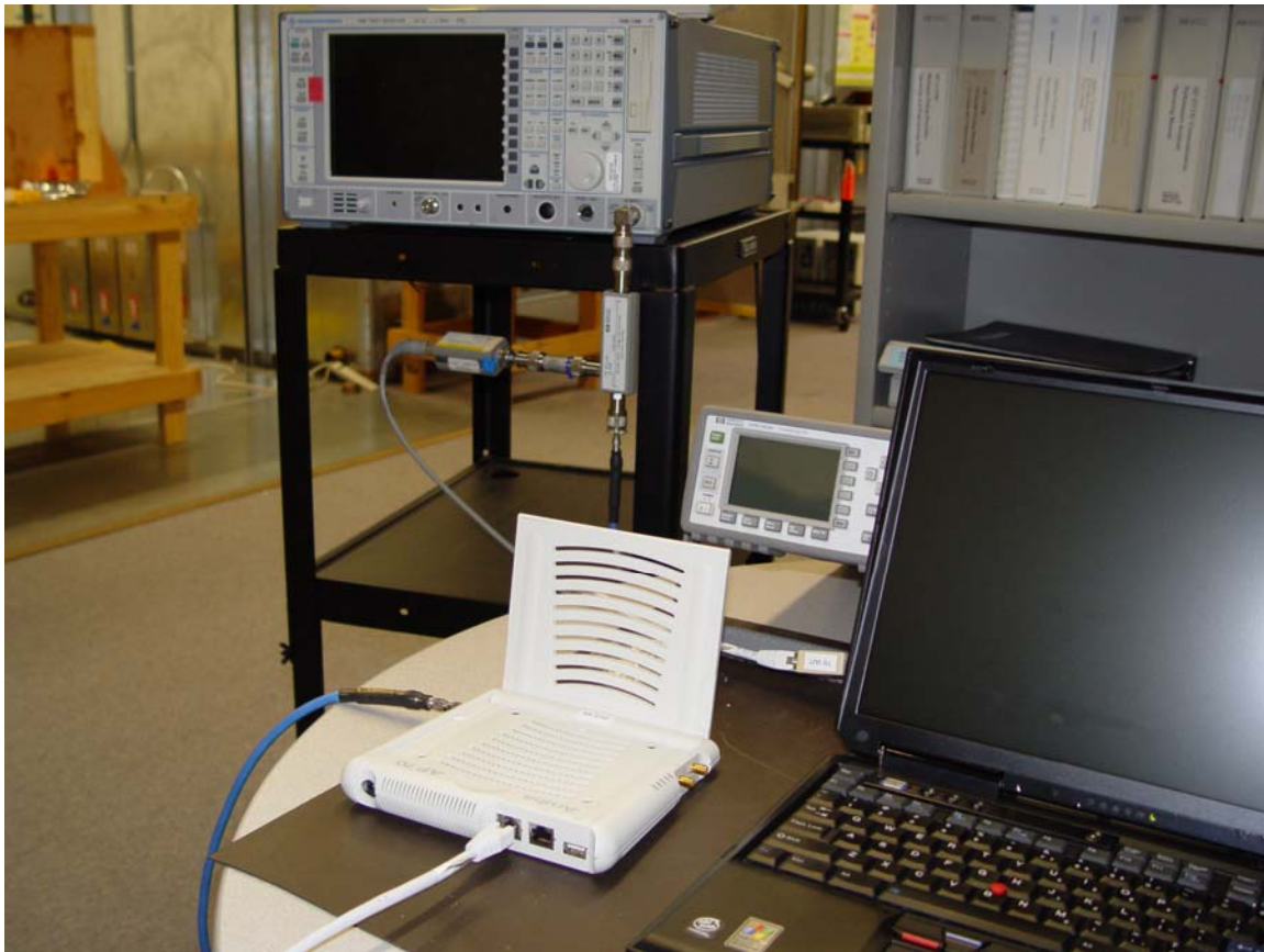
AP70 Wireless Access Point – General Test Setup
