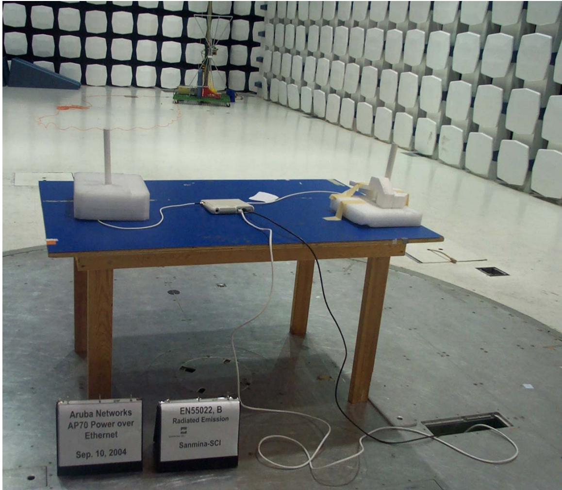
AP70 Wireless Access Point – POE emissions below 1GHz
