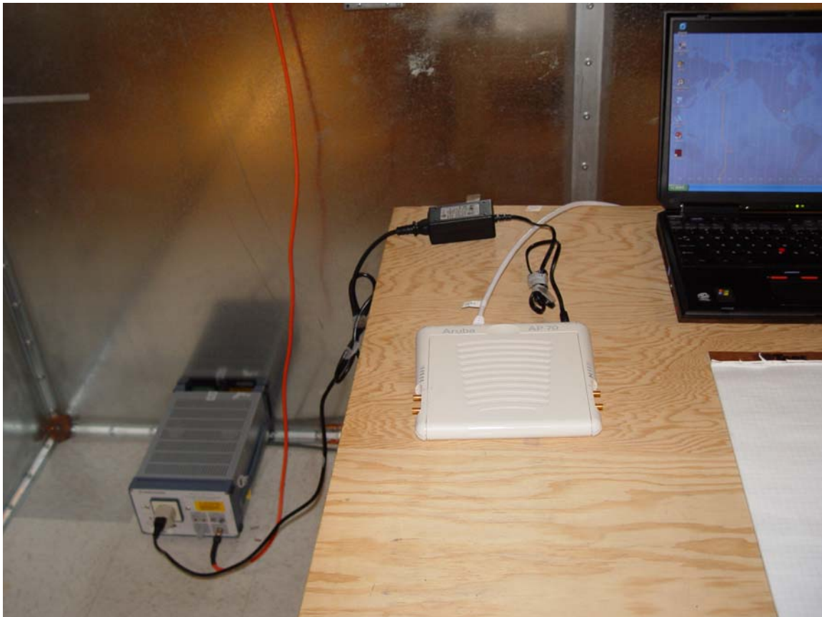
AP70 Wireless Access Point – Conducted Emission Test Set-Up
