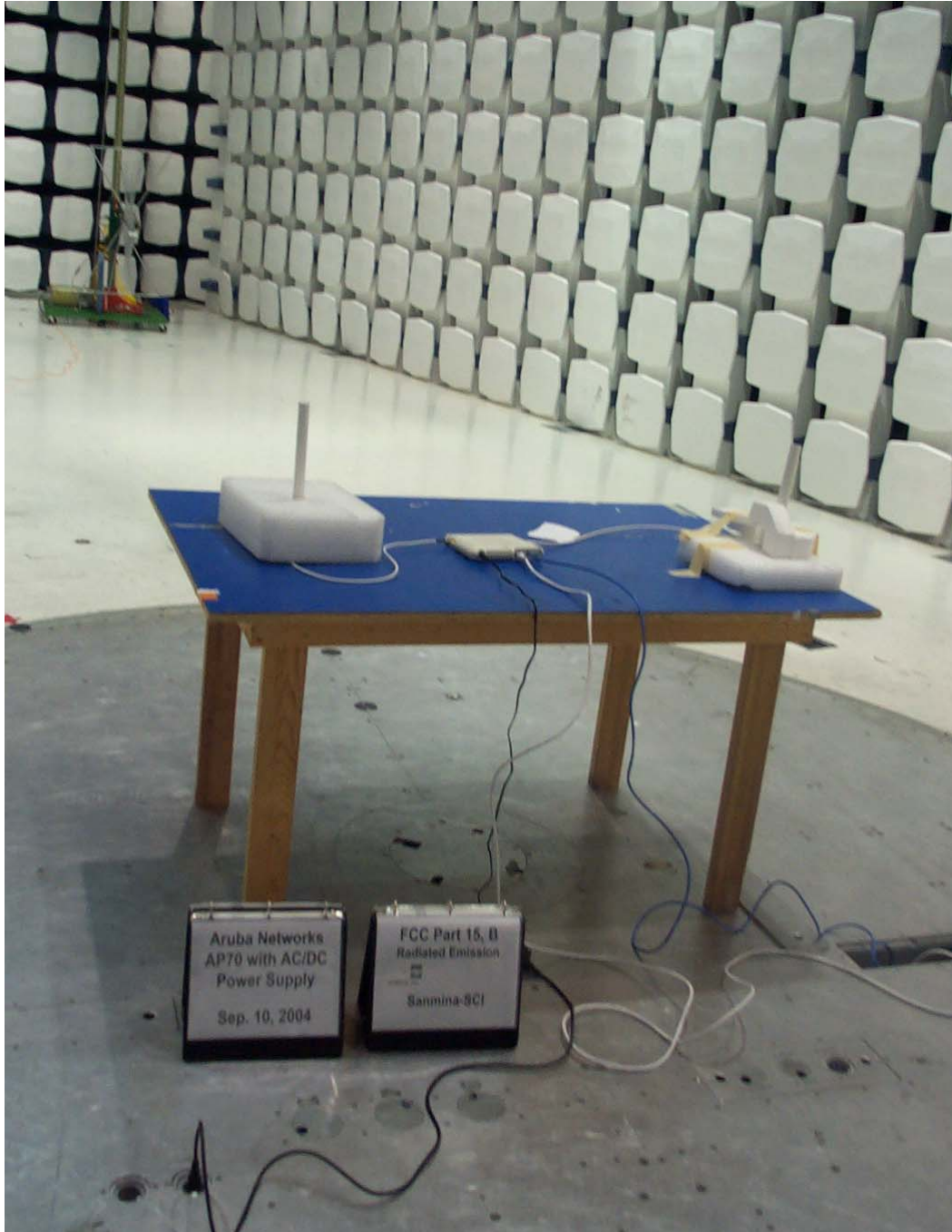
AP70 Wireless Access Point – AC/DC Converter emissions below 1GHz
