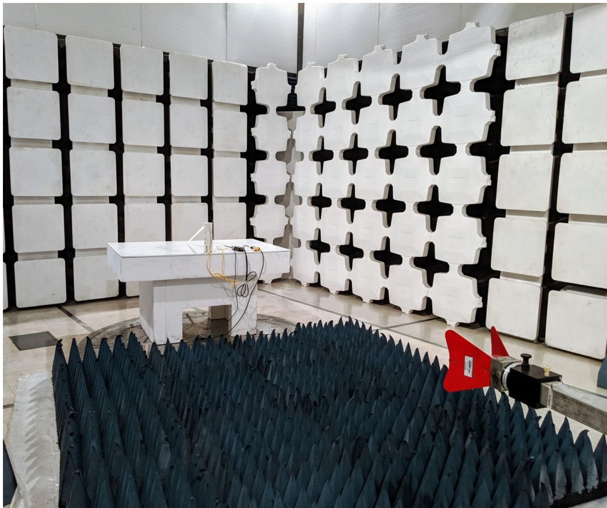
PoE Digital Emissions 1-6GHz
