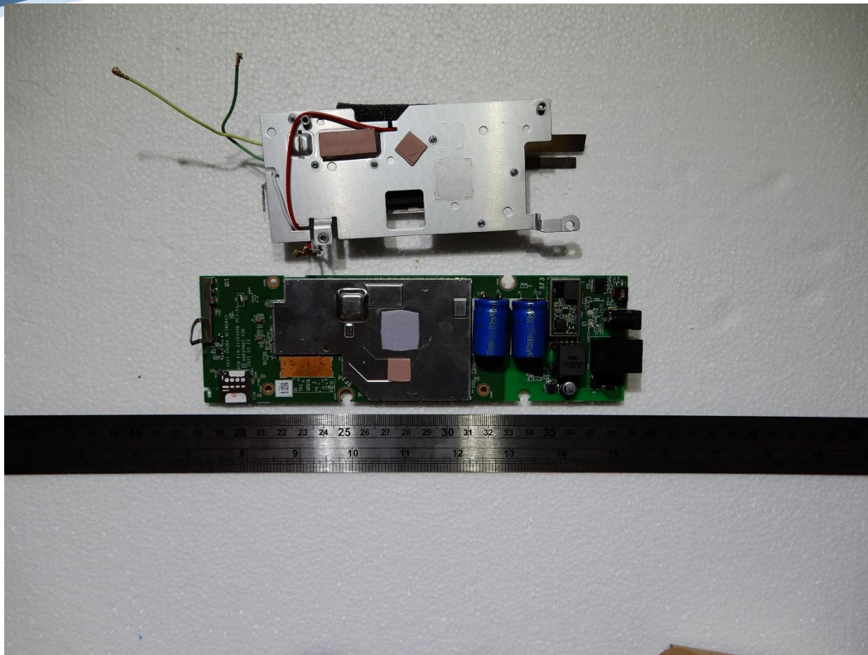
Top View Heatsink Removed
