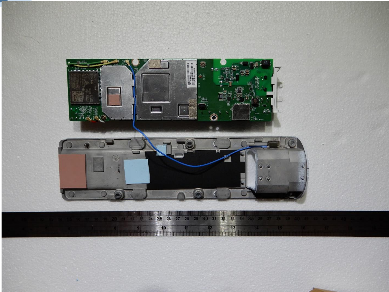
Bottom View With Housing
