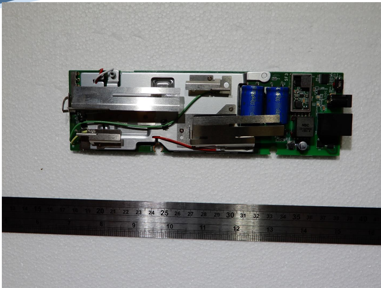
Top View
