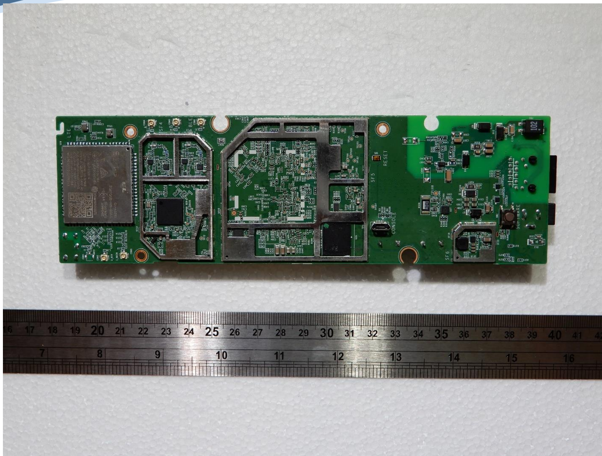
Bottom View Shields Removed
