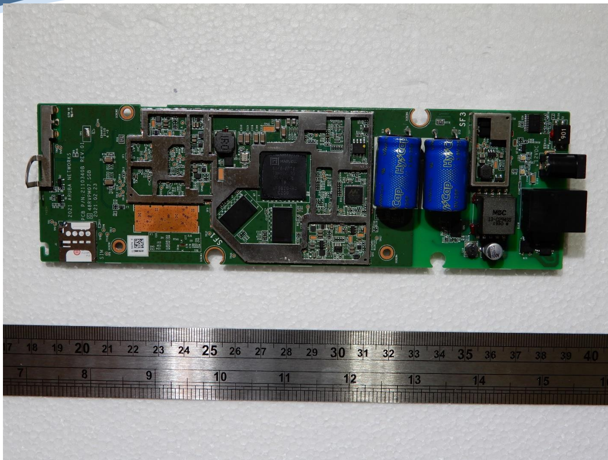
Top View Shield Removed
