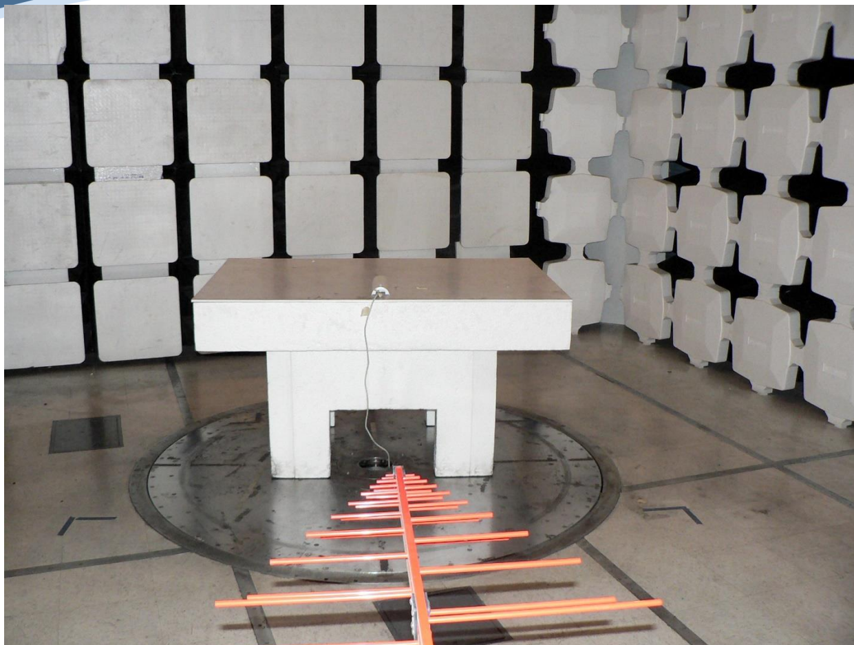
HPEN155 ASIN0304 POE Digital Emissions 30-1000MHz
