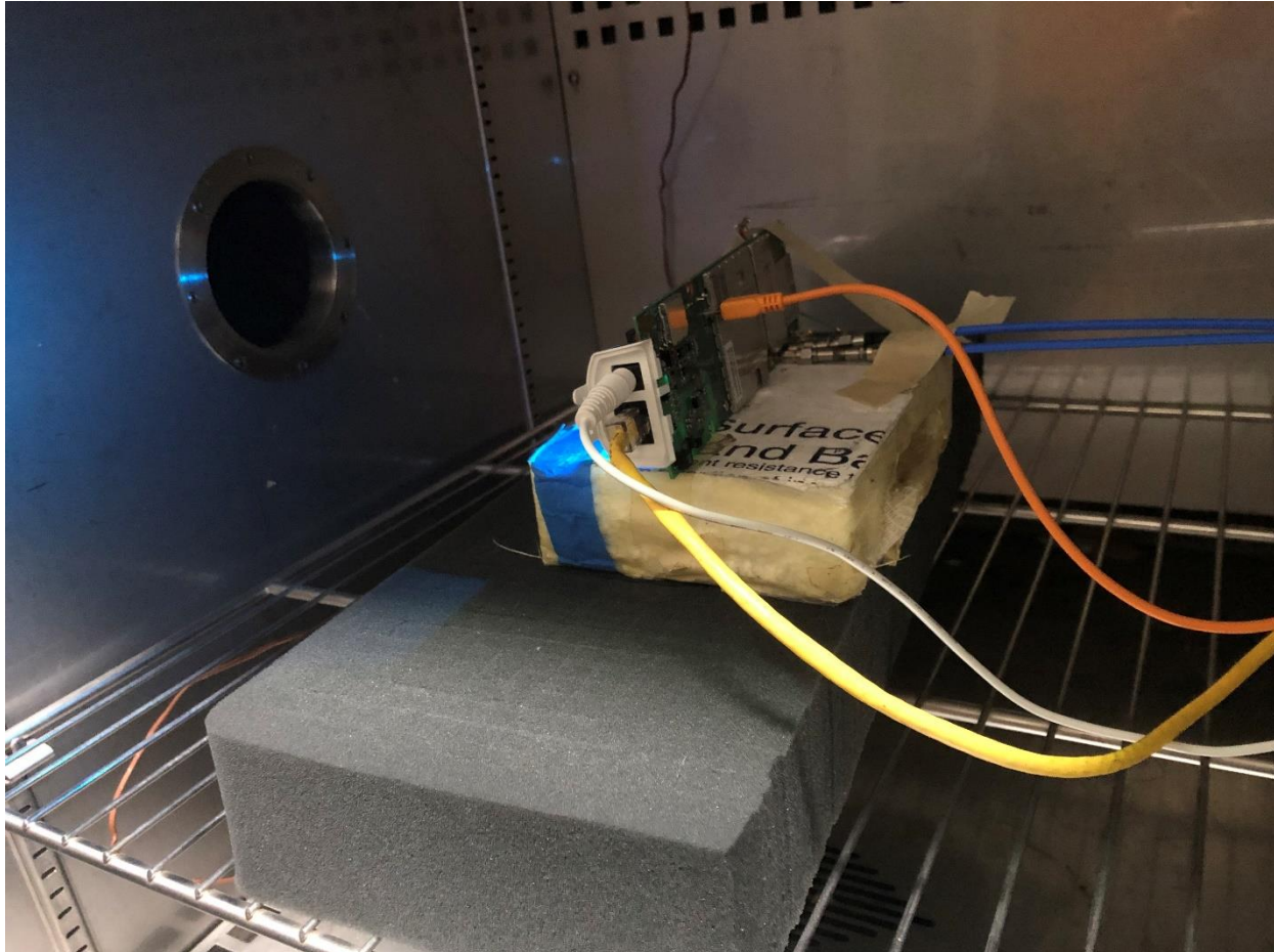
RF Conducted Test Setup 1
