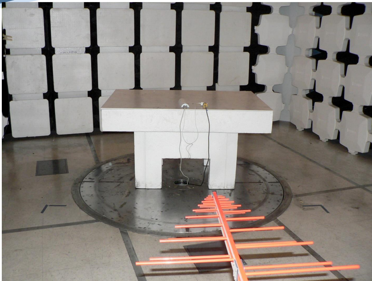
HPEN155 ASIN0304 PS Digital Emissions 30-1000MHz
