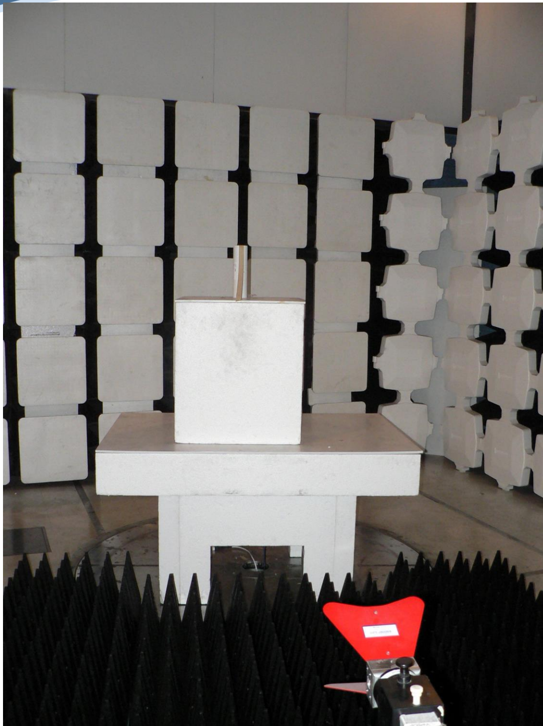
HPEN155 ASIN0304 TX Spurious 1-18GHz
