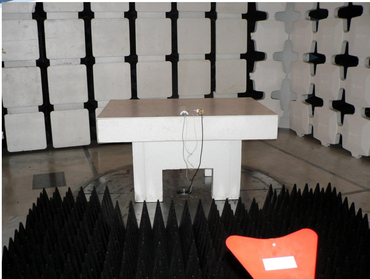
HPEN155 ASIN0304 PS Digital Emissions 1-6GHz
