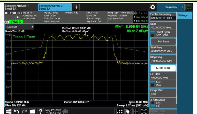
Channel 209 (6995MHz)
