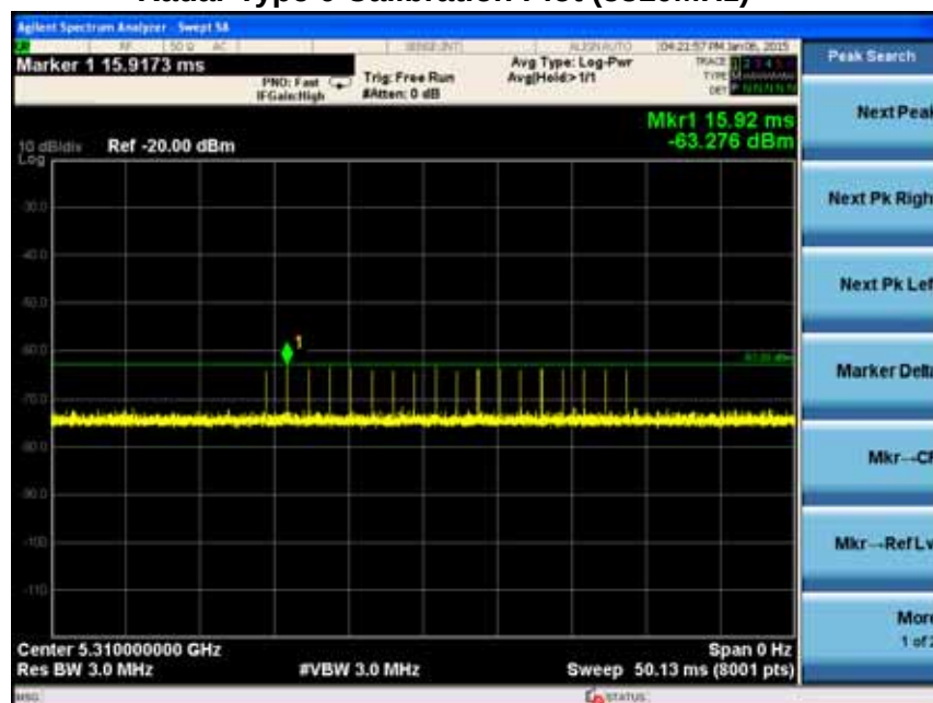
Radar Type 0 Calibration Plot (5310MHz)
