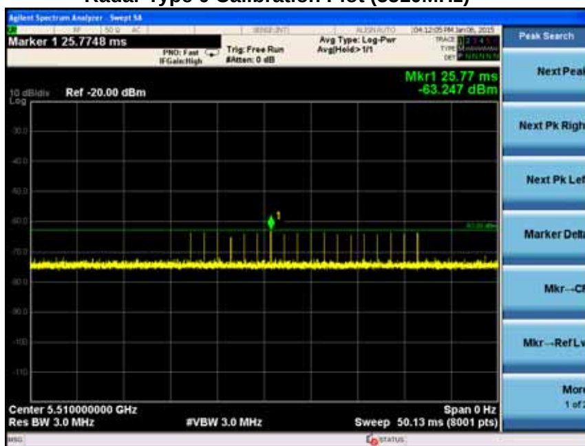
Radar Type 0 Calibration Plot (5510MHz)
