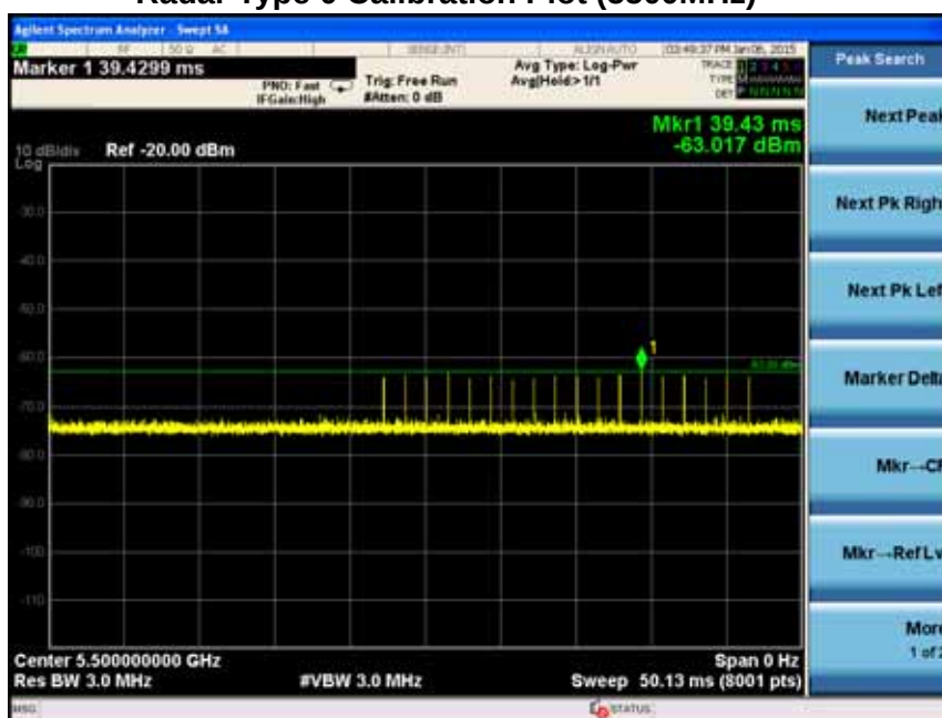
Radar Type 0 Calibration Plot (5500MHz)
