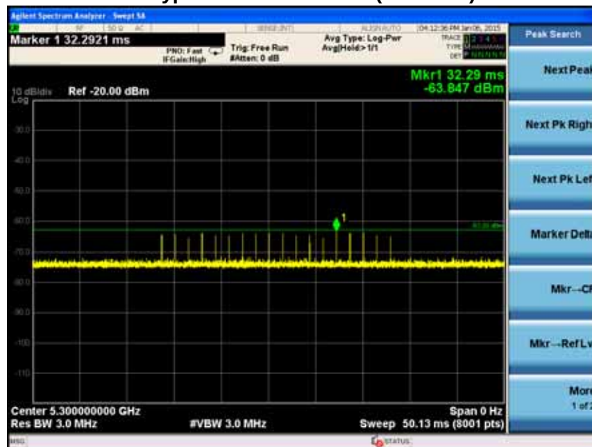
Radar Type 0 Calibration Plot (5300MHz)
