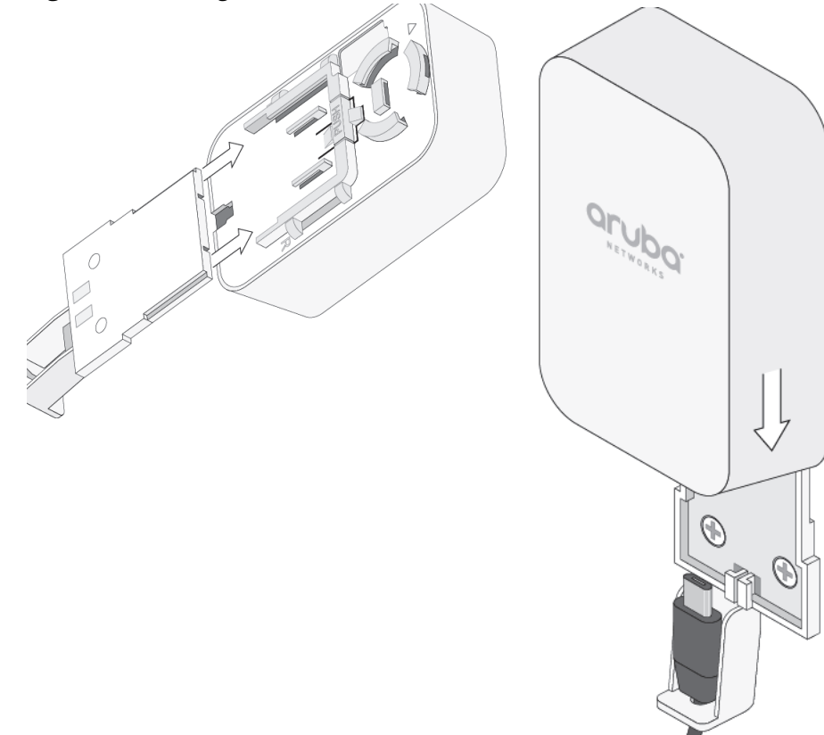
Figure 8 Attaching LS-100 to the Wall Mount Bracket
