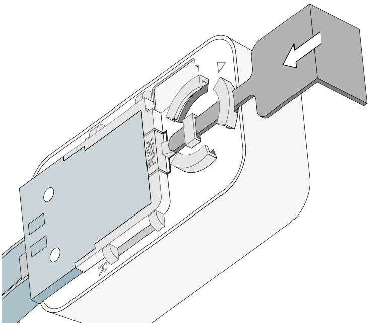
Figure 9 Removing LS-100 from the Wall Mount Bracket
