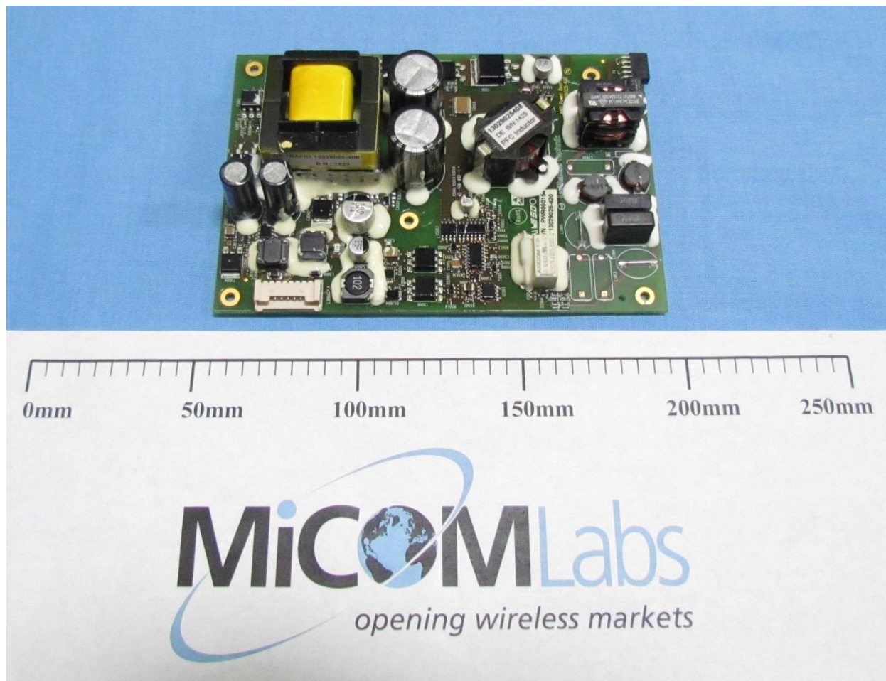
Topside - Power Board P/N: 13029025-420
