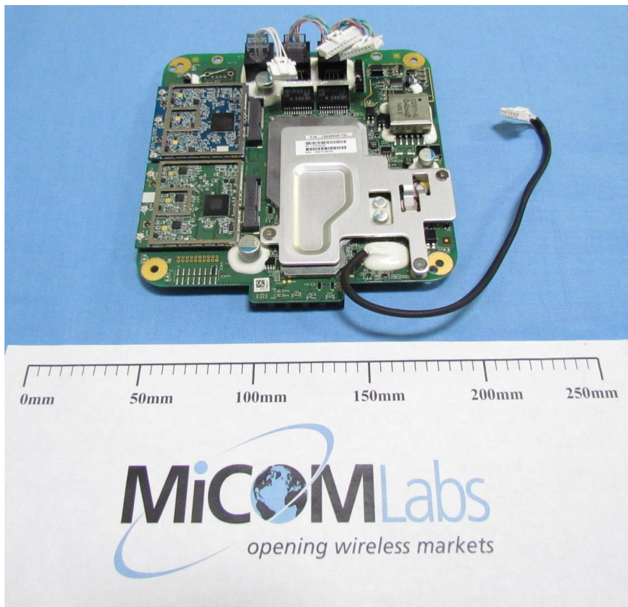
Topside - Radio-Board P/N: 13029025-701
