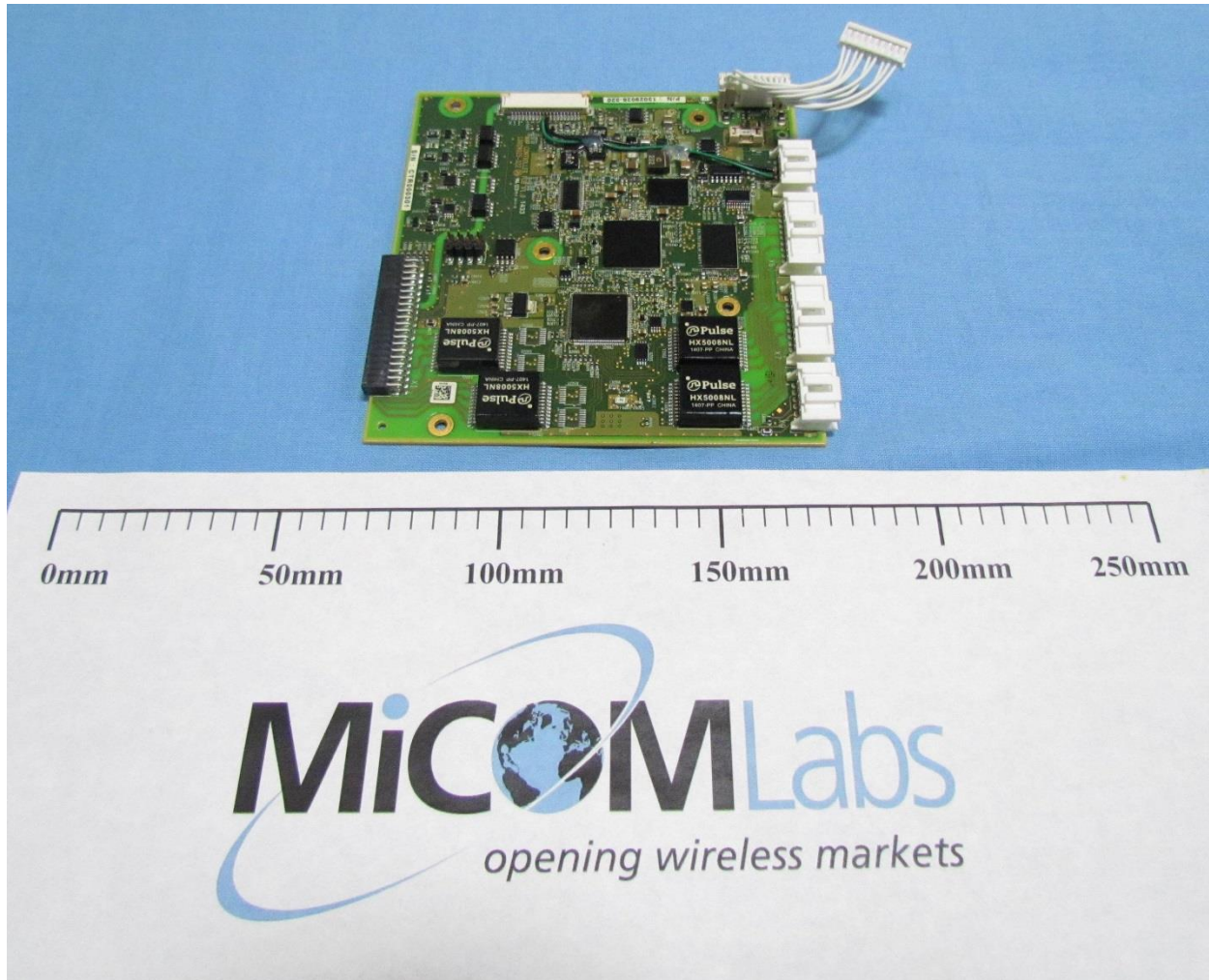
Topside - Controller Board P/N: 13029025-320
