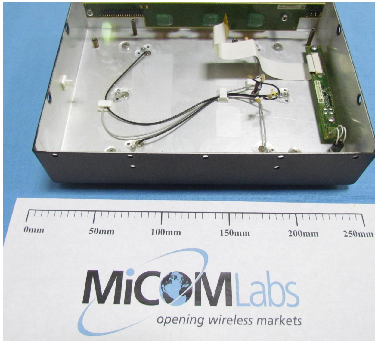
Internal assembly - Connector-Board / LED-Board / Antenna-Wiring
