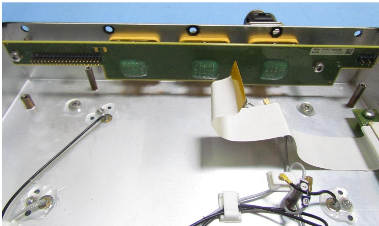
Internal assembly - Connector-Board / Flex-Cable
