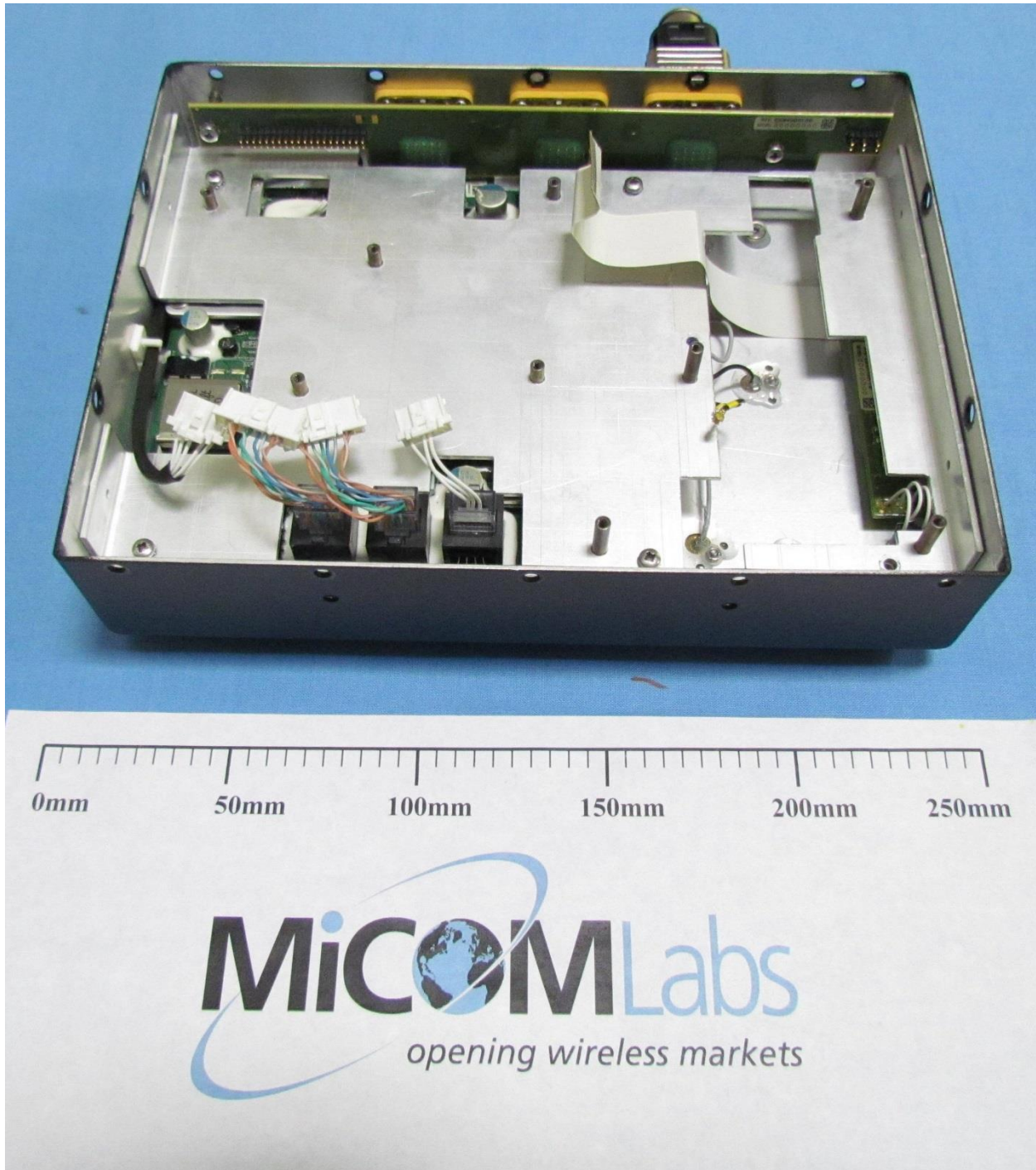
Internal assembly - Connector-Board / Heatsink with installed Radio-Board (P/N:13029025-701)
