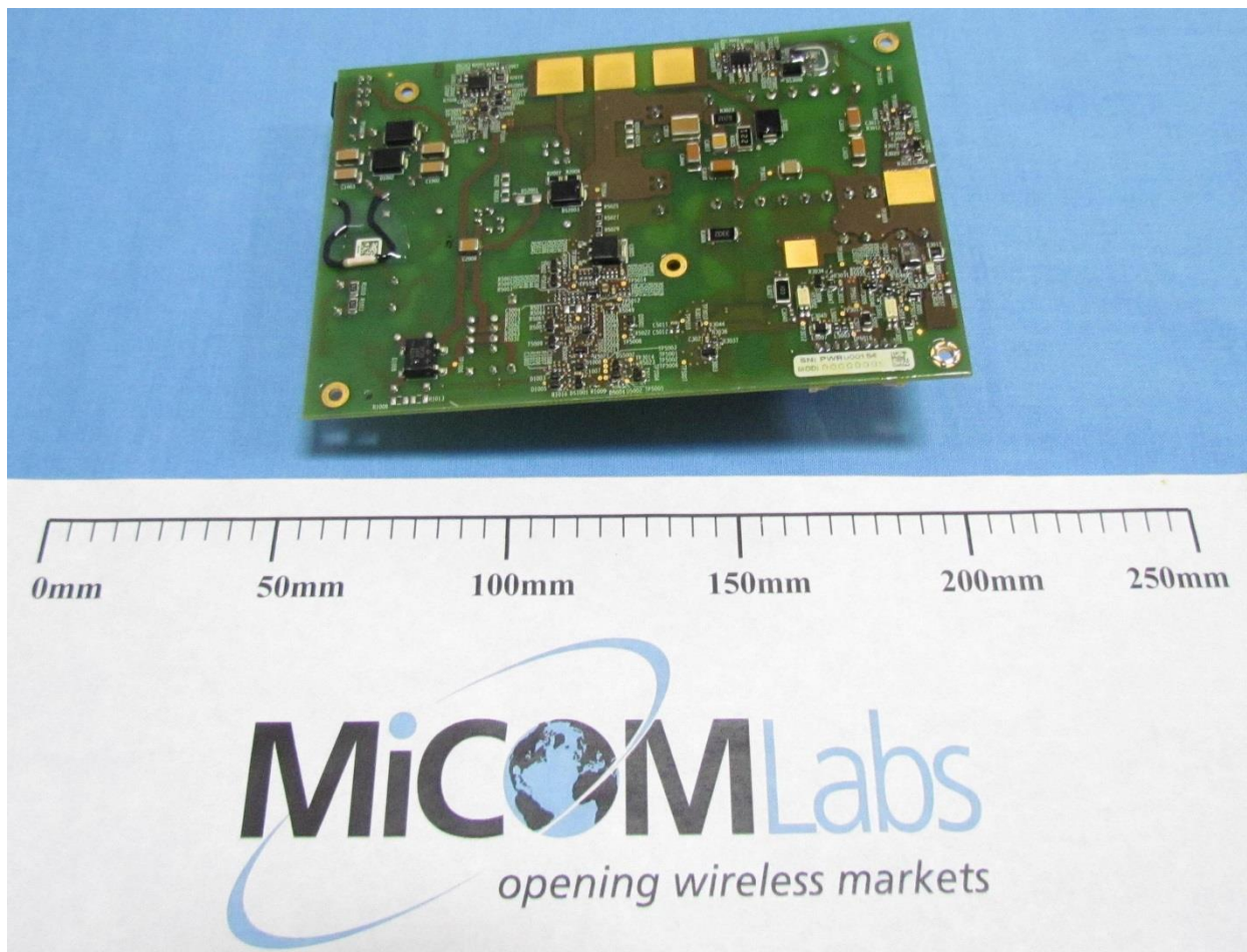
Bottomside - Power Board P/N: 13029025-420
