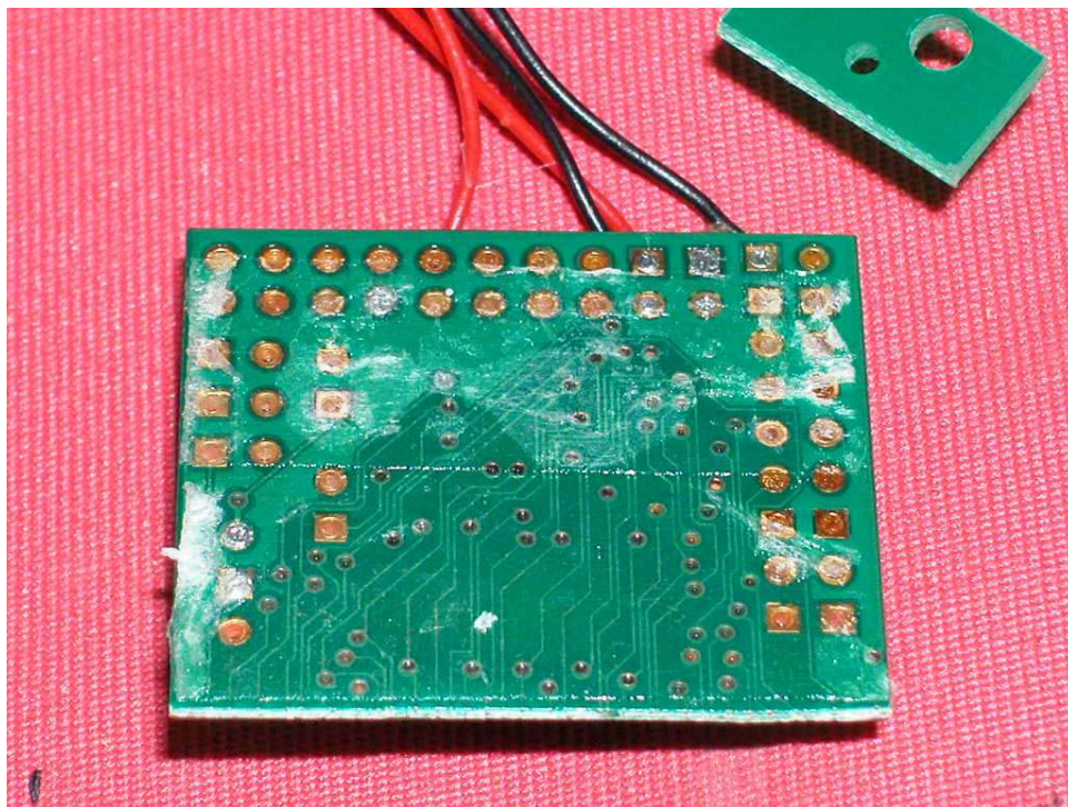
Handset MCU PCB solder side
