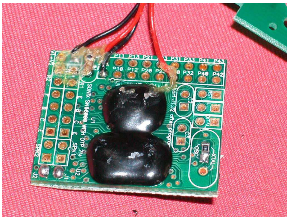
Handset MCU PCB comp side
